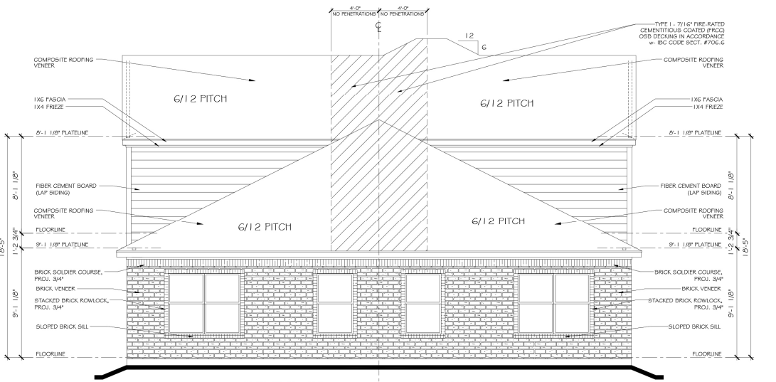
(UNIT 2) (UNIT 1) REAR ELEVATION "B" SCALE: 1/4" = 1'-0" (22"x34" SHEET) 1/8" = 1'-0" (11"x17" SHEET)
