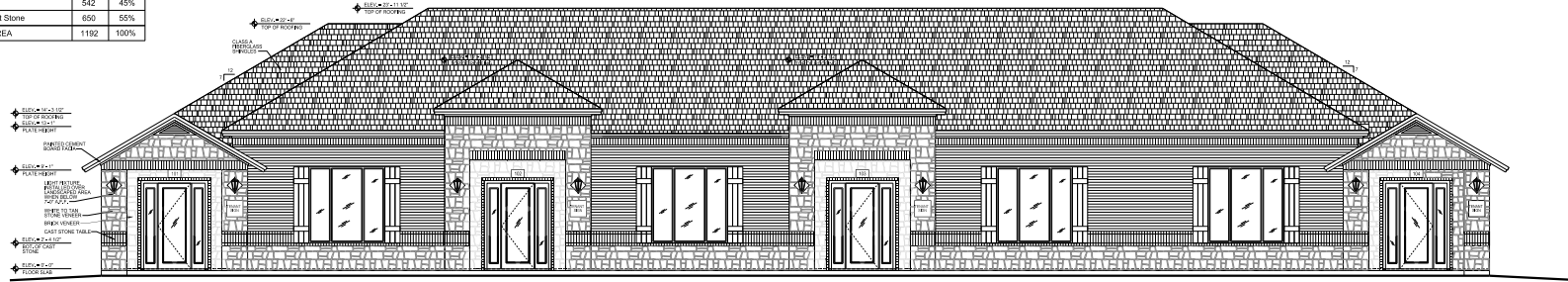
01 East Elevation
