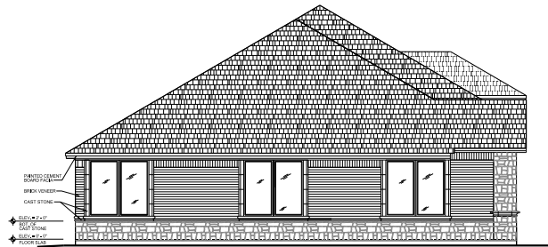
02 South Elevation
