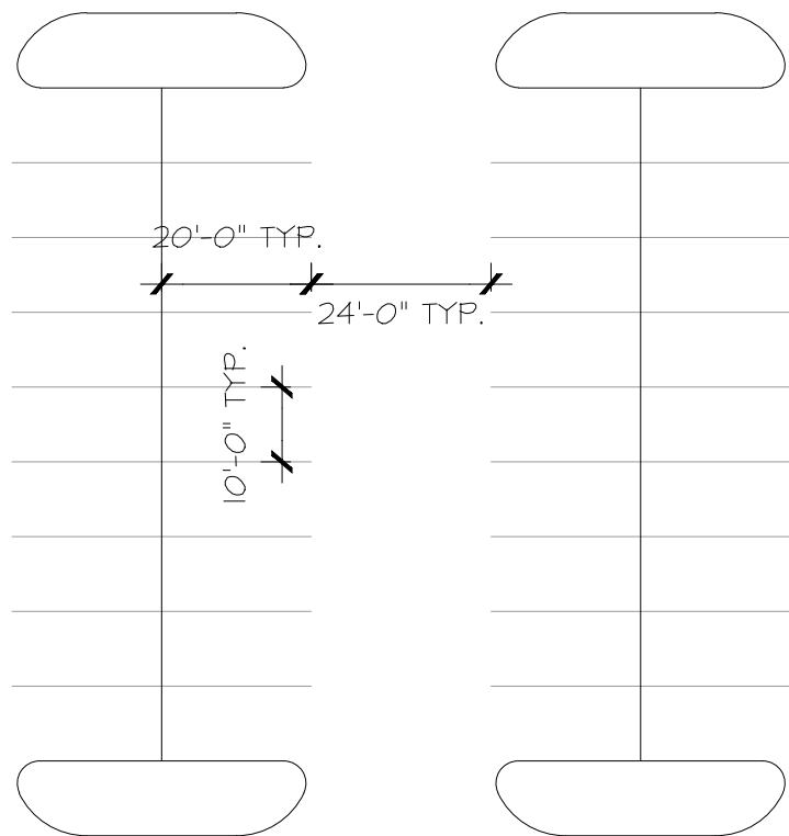
90 DEGREE PARKING
