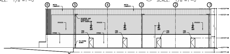
EAST ELEVATION SCALE: 1/8"=1'-0"
