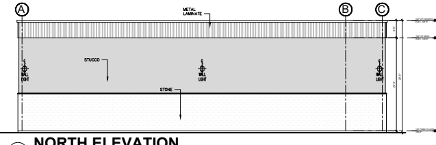
NORTH ELEVATION SCALE: 1/8"=1'-0"
