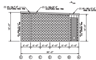
ENDWALL SHEETING ELEVATION @ COLUMN LINE 1 BUILDING 1 - SCALE: 3/16" = 1'-0"
