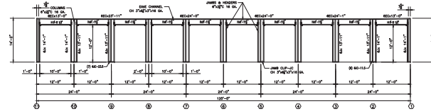
SIDEWALL FRAMING ELEVATION @ COLUMN LINE C BUILDING 2 - SCALE: 1/8" = 1'-0"
