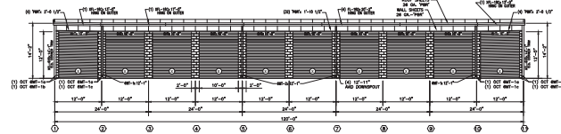
SIDEWALL SHEETING ELEVATION @ COLUMN LINE A BUILDING 2 - SCALE: 1/8" = 1'-0"
