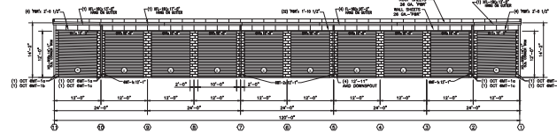
SIDEWALL SHEETING ELEVATION @ COLUMN LINE C BUILDING 2 - SCALE: 1/8" = 1'-0"
