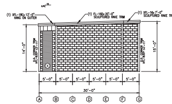
ENDWALL SHEETING ELEVATION @ COLUMN LINE 11 BUILDING 1 - SCALE: 3/16" = 1'-0"
