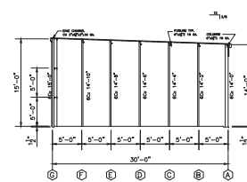
CROSS SECTION @ COLUMN LINES 2-9 BUILDING 1 - SCALE: 3/16" = 1'-0"
