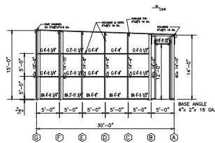
ENDWALL FRAMING ELEVATION @ COLUMN LINE 1 BUILDING 1 - SCALE: 3/16" = 1'-0"
