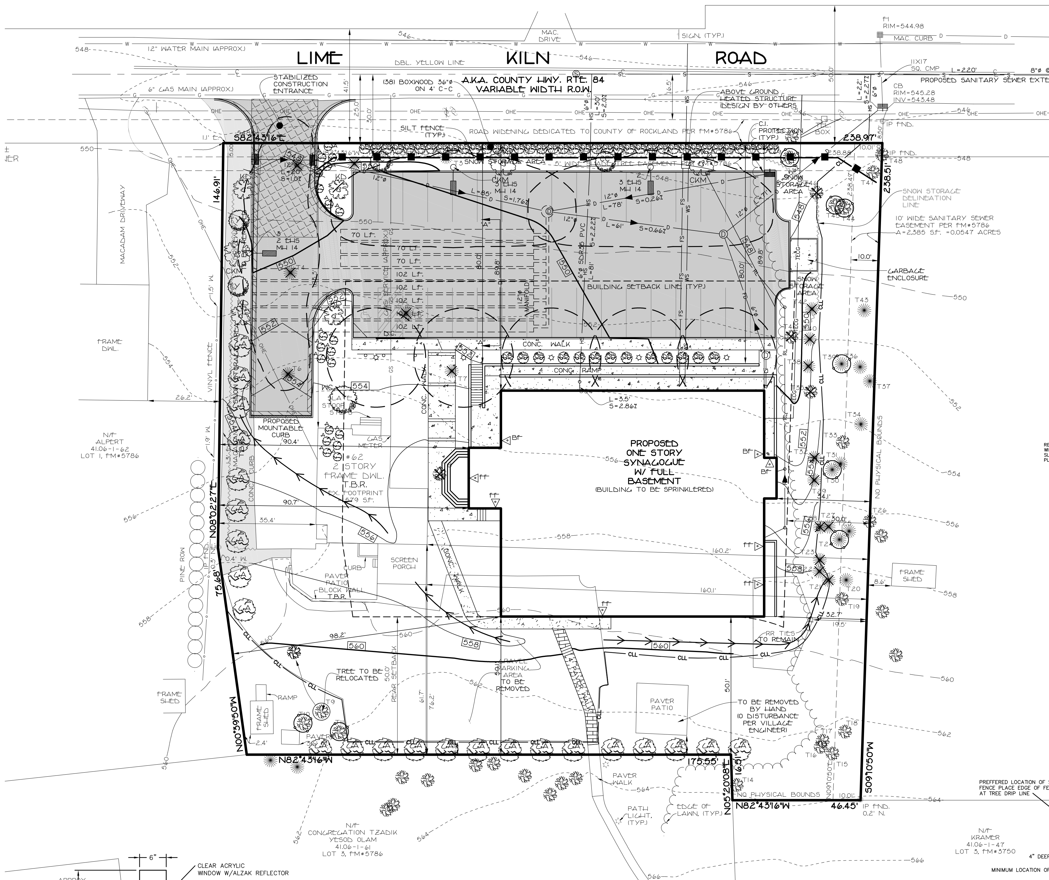
N.T.S. NOTE: LIGHT HEADS SHALL BE ADJUSTED AND CUT-OFFS INSTALLED TO PREVENT LIGHT FROM PROJECTING ON TO NEIGHBORING PROPERTIES AND R.O.W.
