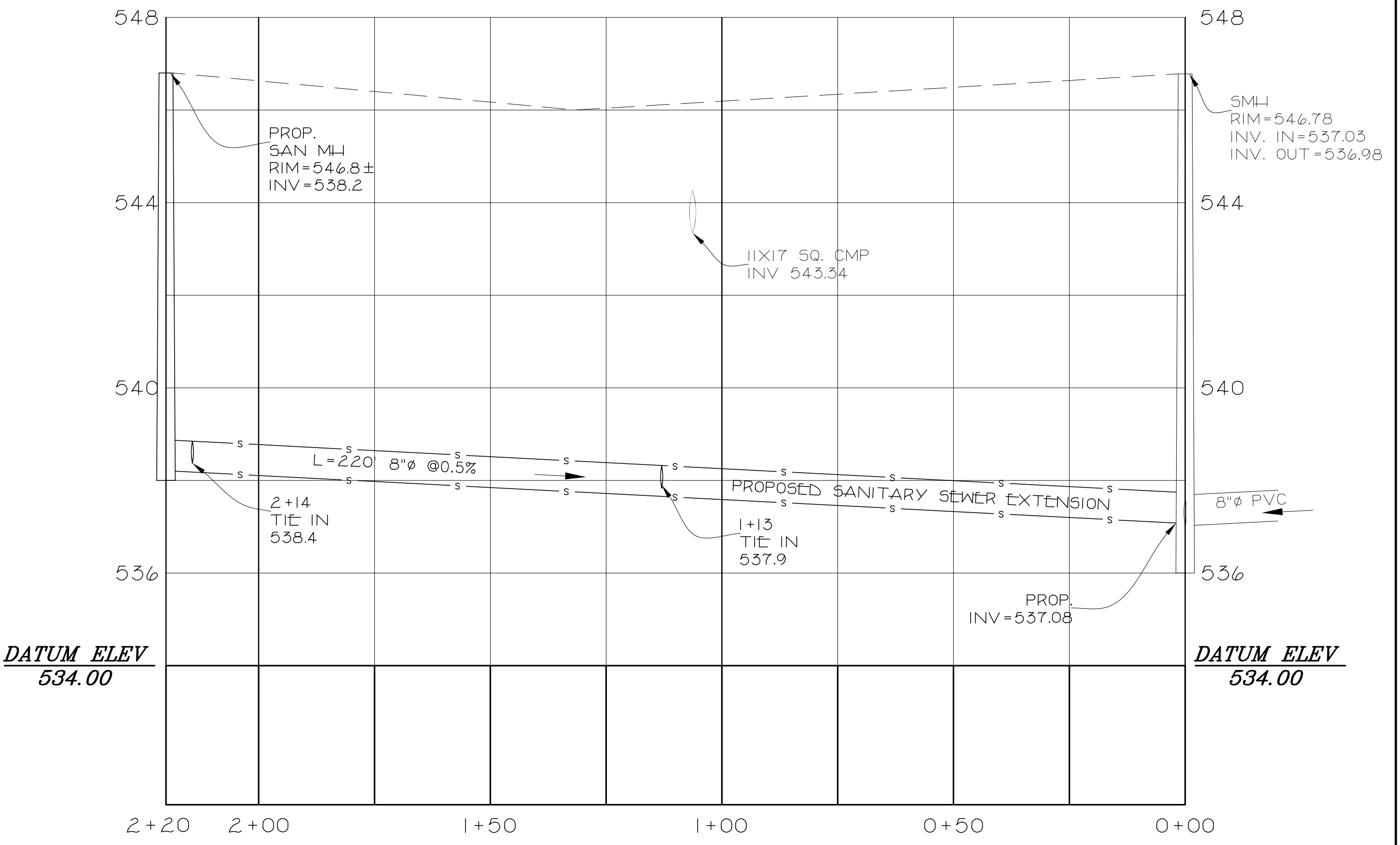
SEWER PROFILE IN LIME KILN ROAD SCALE: H-1"=20', V-1"=2'
