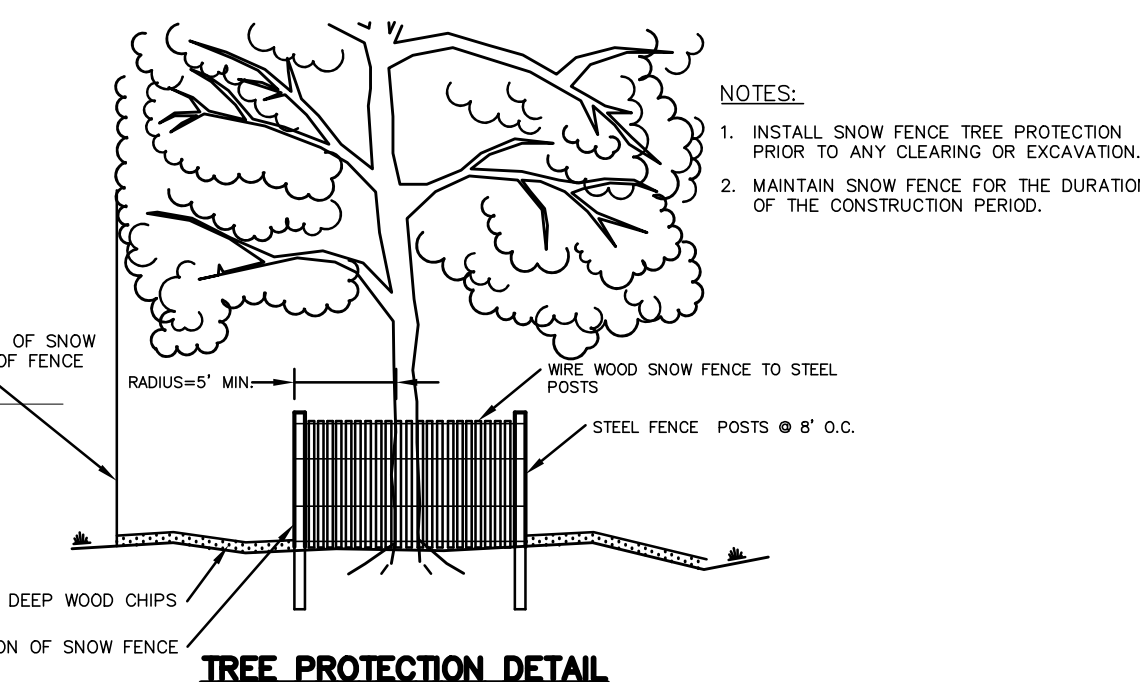
TREE PROTECTION DETAIL
