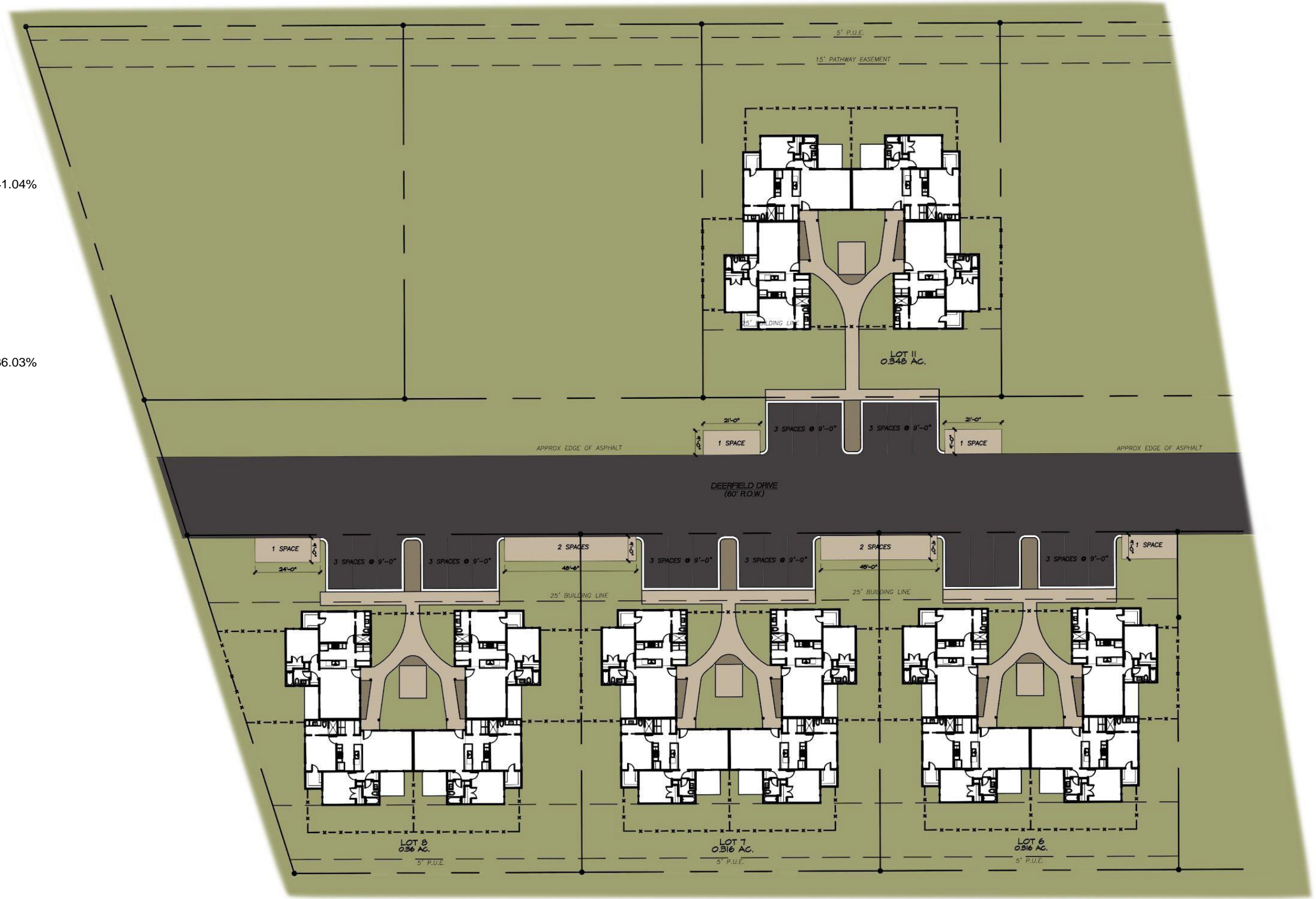
SITE PLAN 1" = 40'-0"
