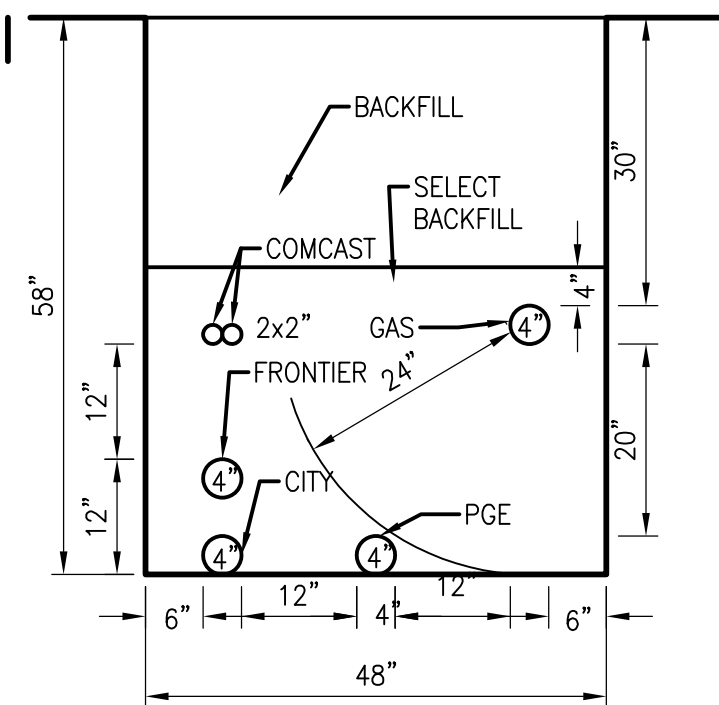
SECTION C
