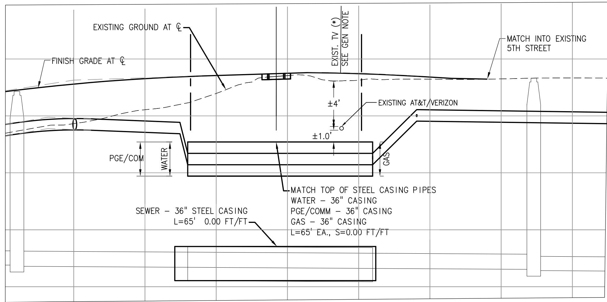
1 BORING PROFILE 63 1" = 10'
