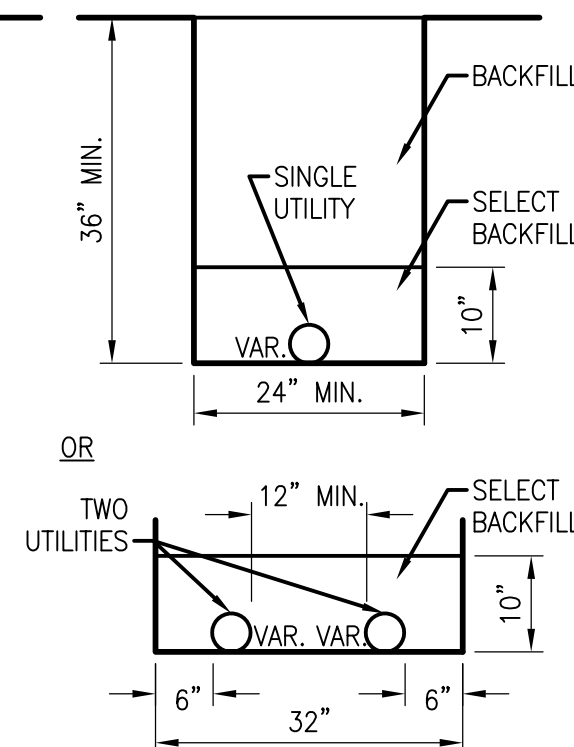
SECTION E
