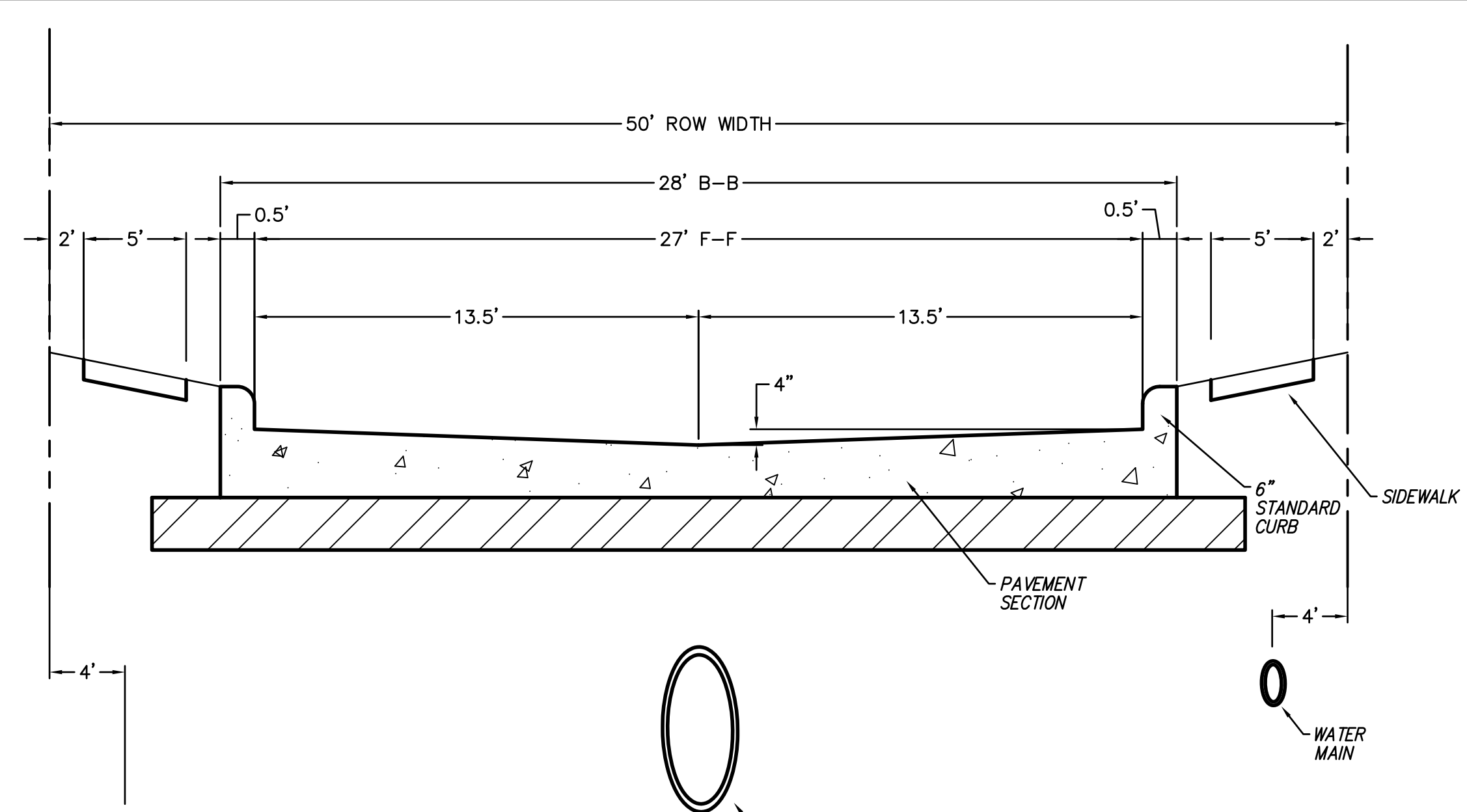
TYPICAL ROW SECTION
