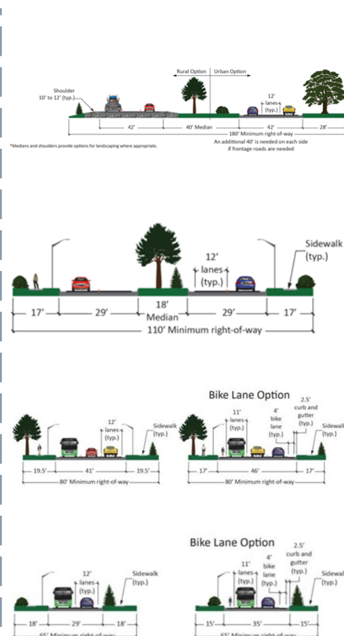
Figure 3.1: Street Cross-sections.
