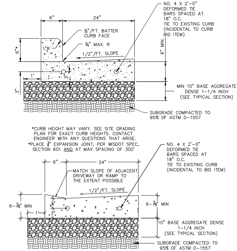
7 30-INCH BARRIER CONCRETE CURB & GUTTER N.T.S.
