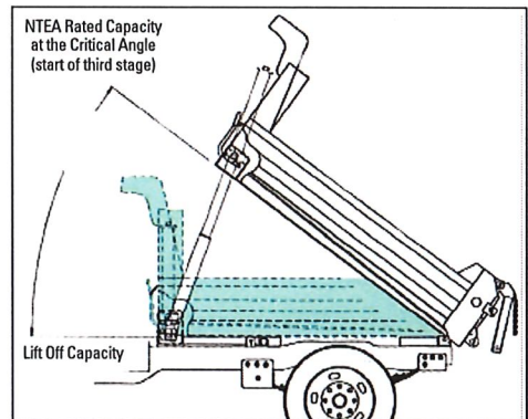
Illustrated above are the NTEA Capacity and Liftoff Capacity point of measure for the hoist.
