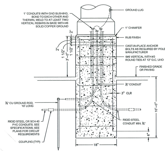
20' LIGHT POLE BASE NOT TO SCALE
