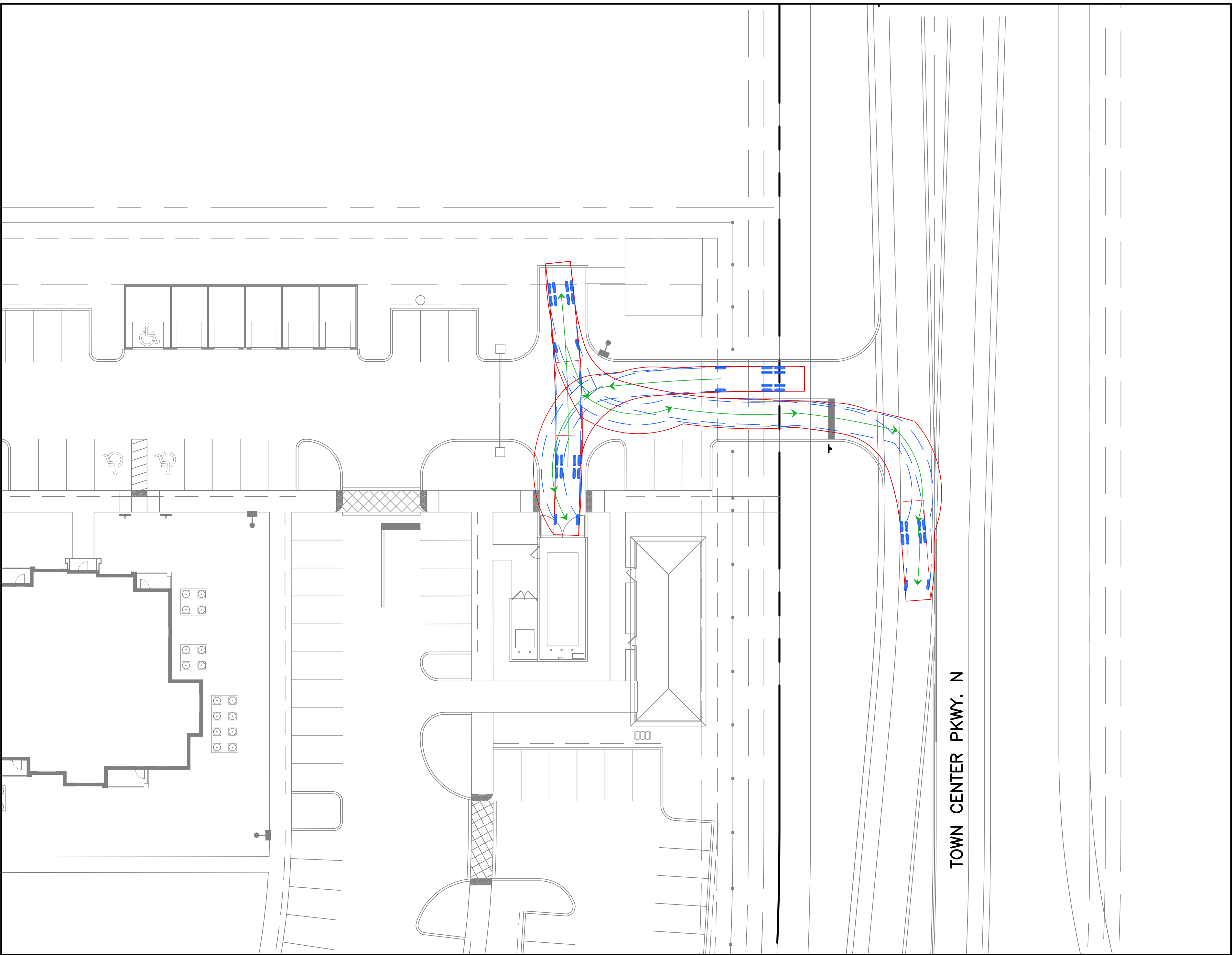
GARBAGE TRUCK
