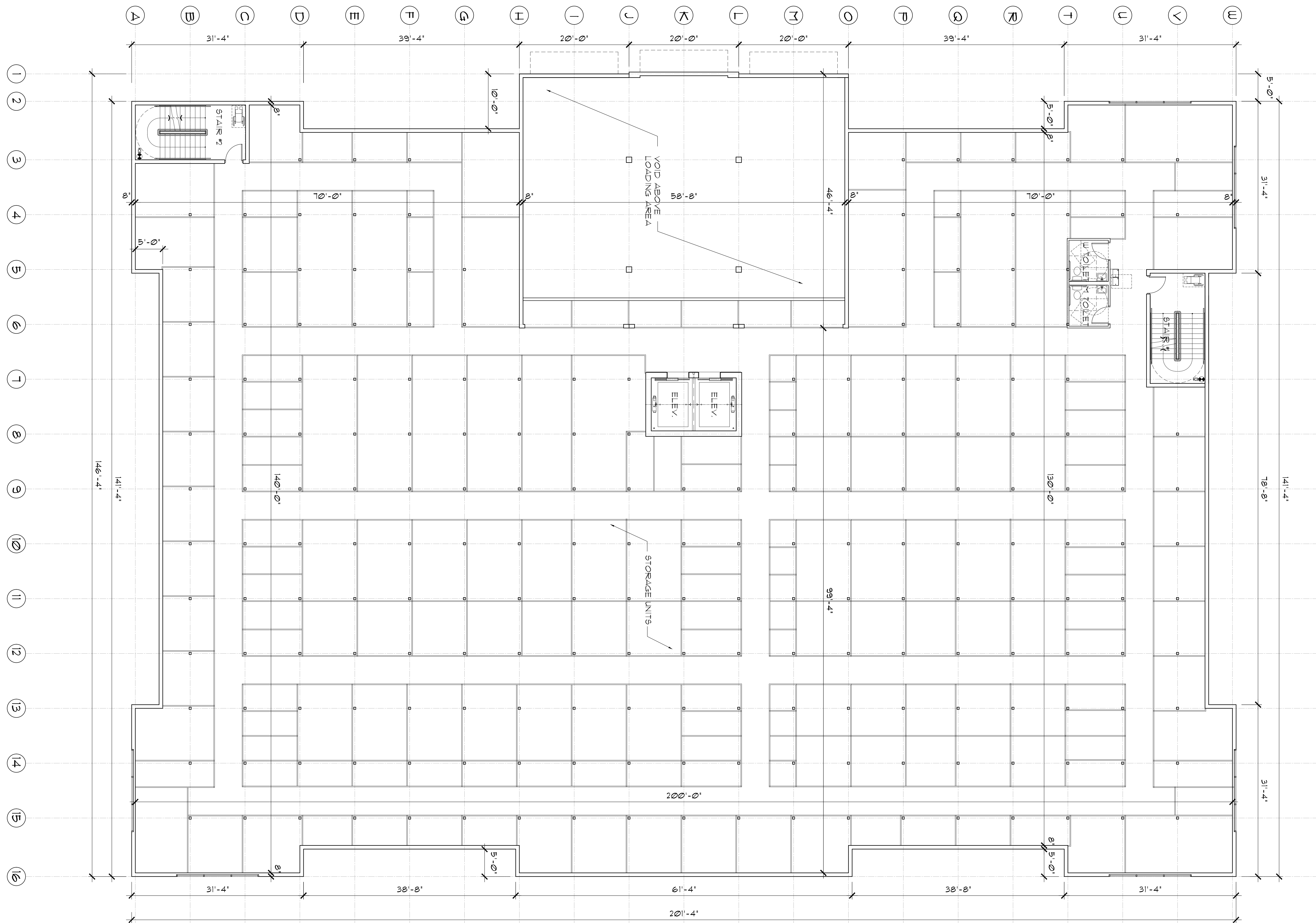
1 A4.1 BUILDING 1 - SECOND FLOOR PLAN 1/8" = 1'-0"
