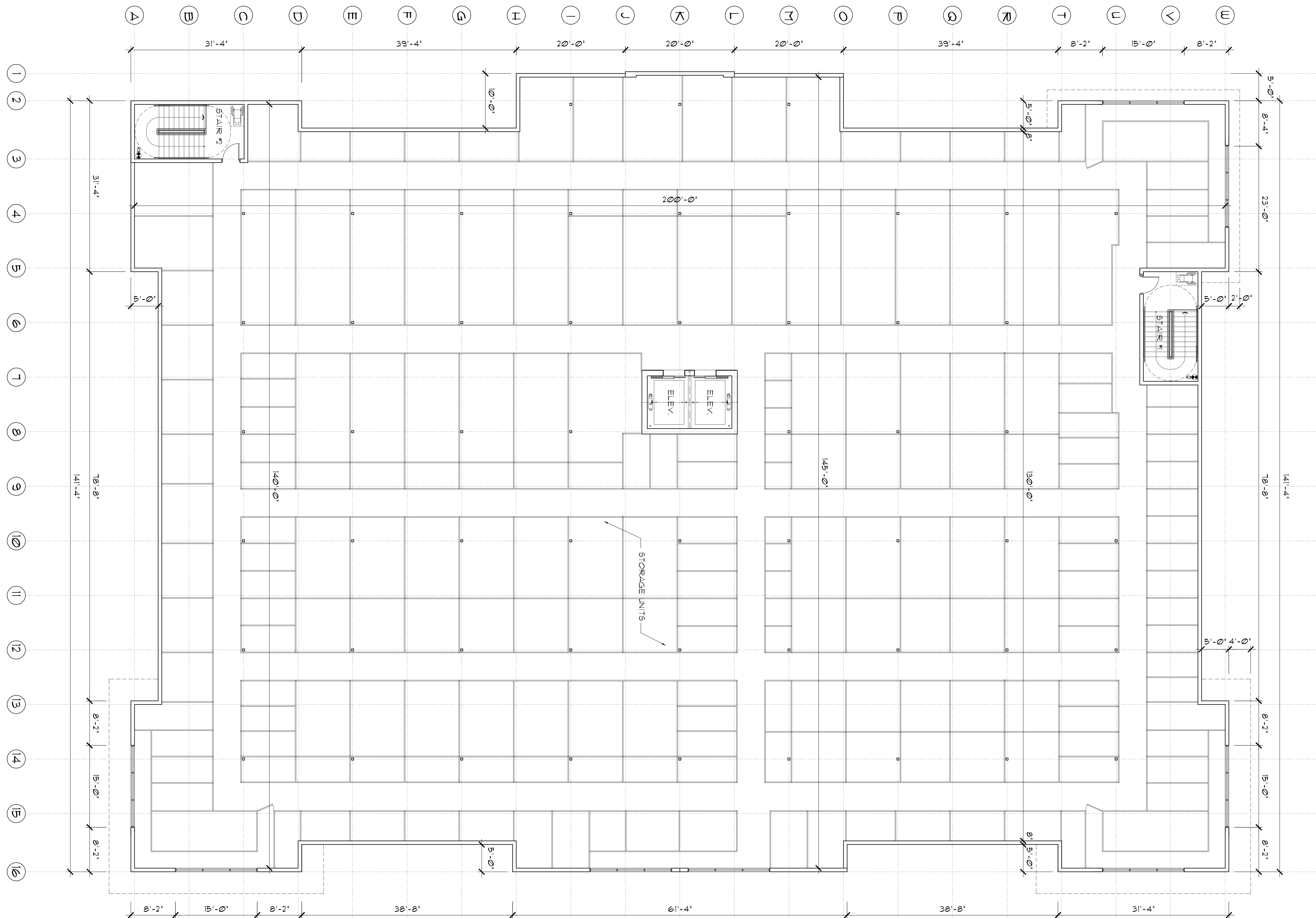
1 A42 BUILDING 1 - THIRD FLOOR PLAN 1/8"=1'-0"
