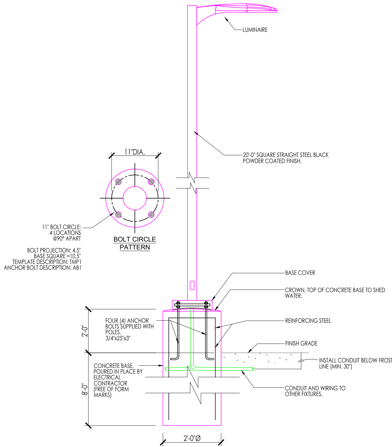
LIGHTING STANDARD ELEVATION (TYPE OP1/OP2)
