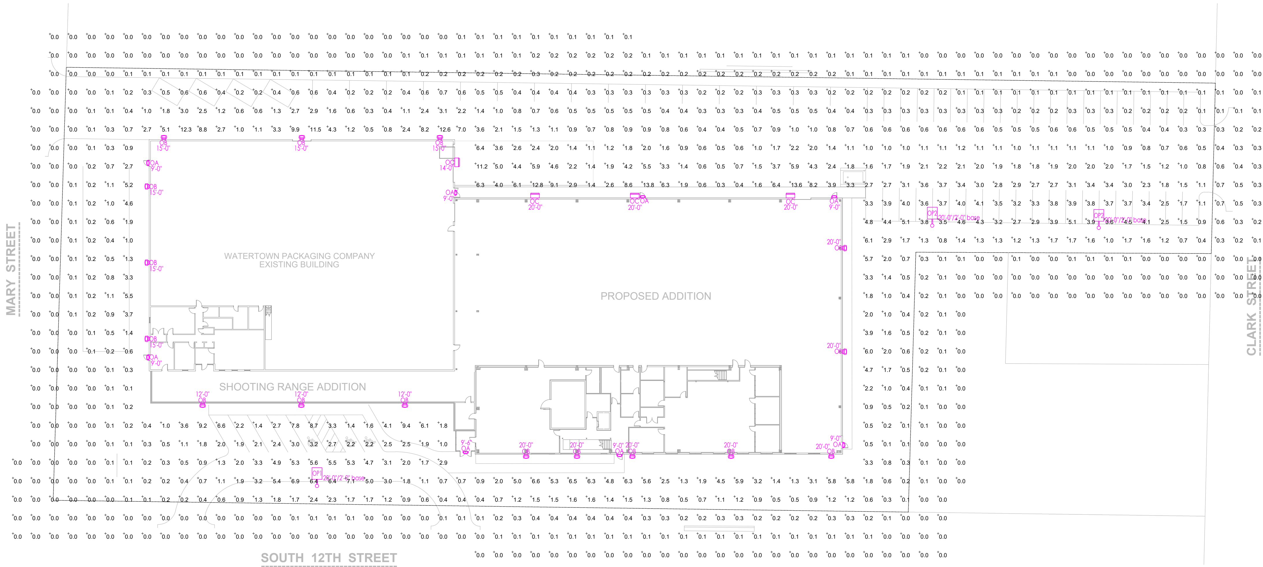
SITE PLAN - PHOTOMETRIC SCALE: 1" = 30'-0"
