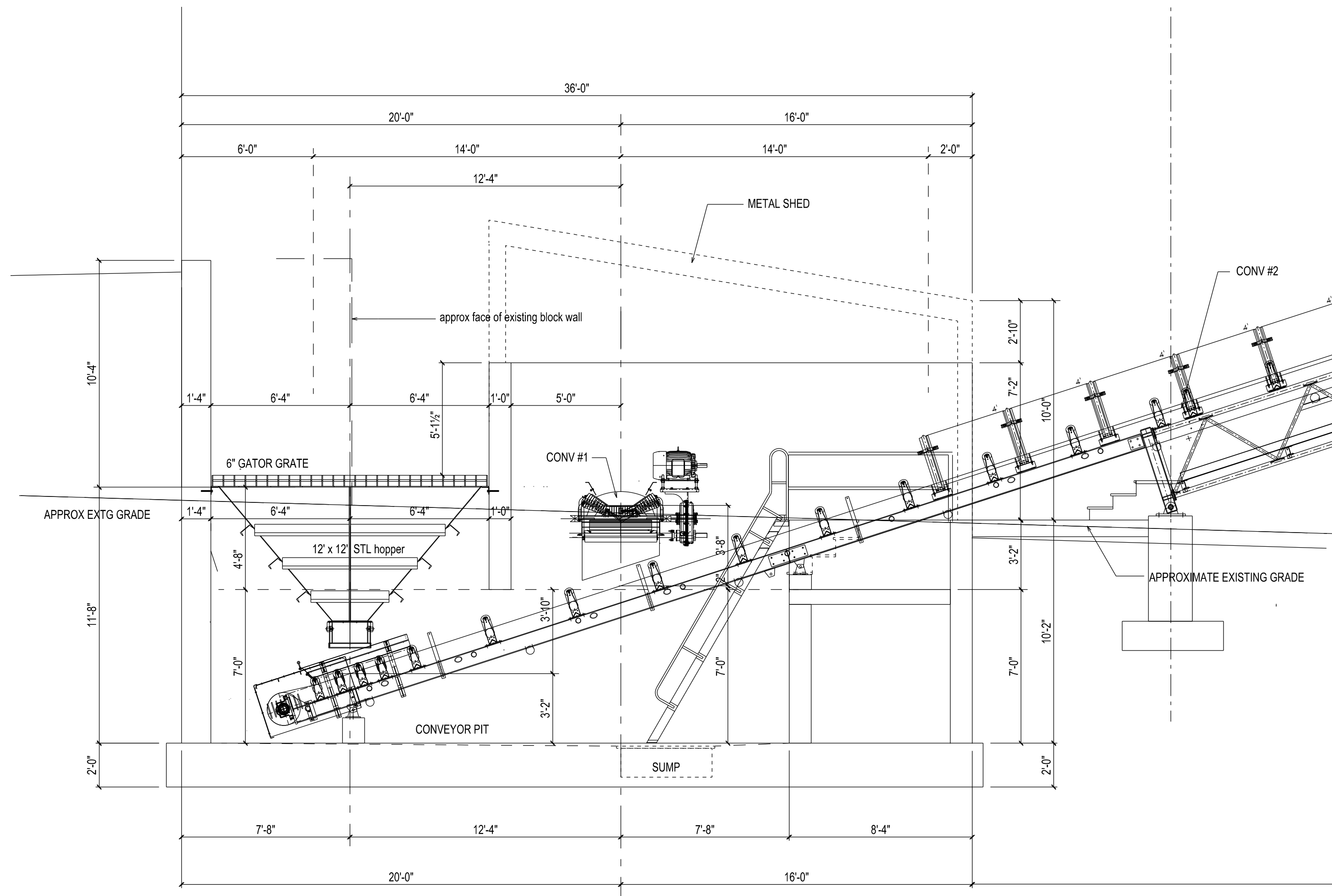
2 BUILDING SECTION @ NORTH END 1/4"=1'-0"
