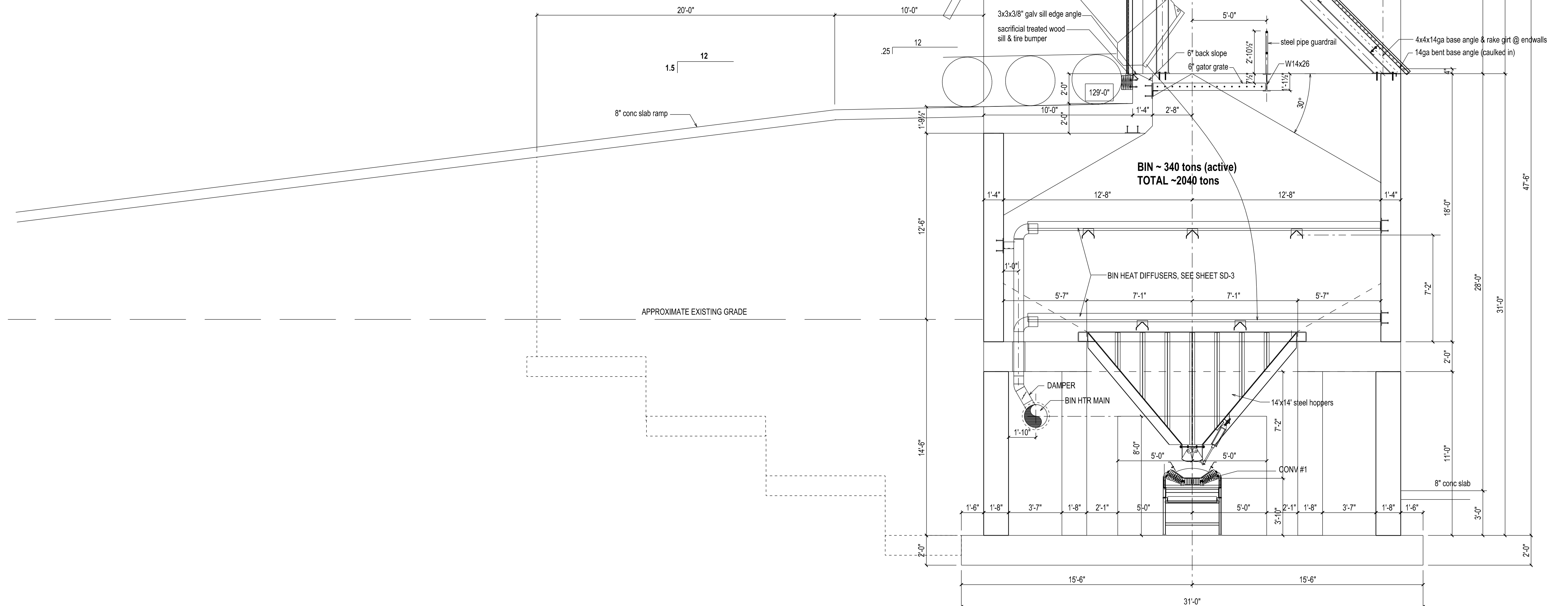
1 BUILDING SECTION @ BINS 1/4"=1'-0"
