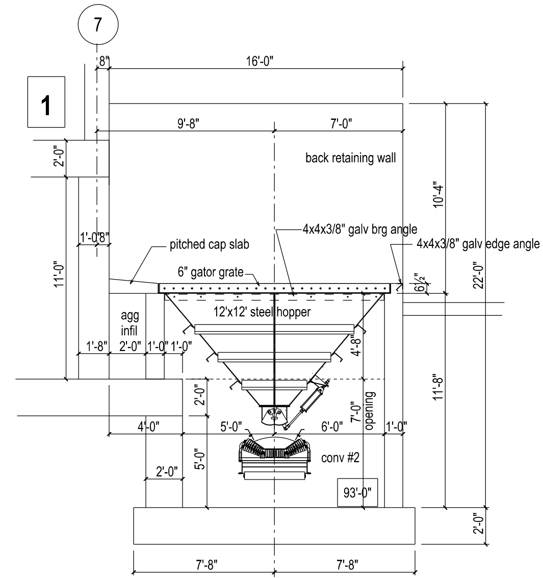
2 BUILDING SECTION @ HOPPER 3/16"=1'-0"
