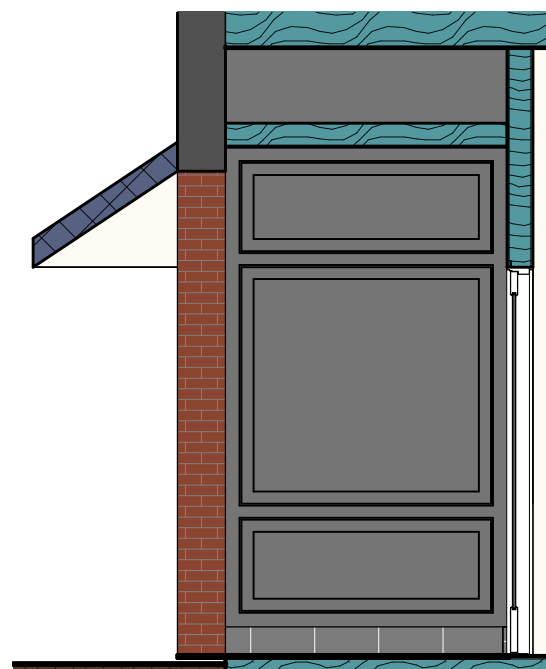
4 Section 3 1/4" = 1'-0"
