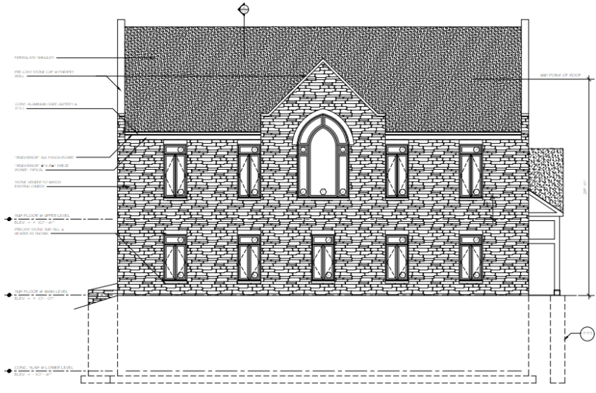
WEST ELEVATION - FACING WINCHESTER STREET - SCHEME B SCALE: 1/8" = 1'-0"
