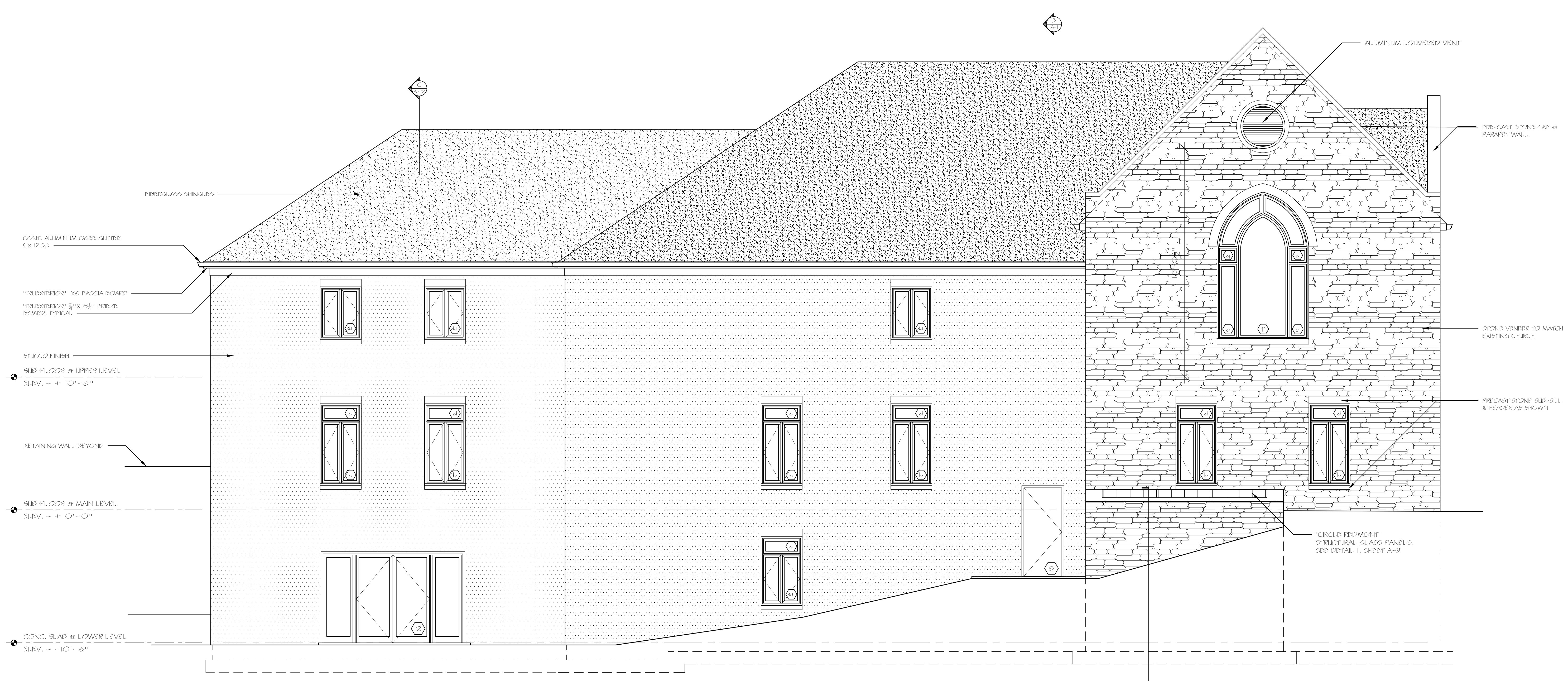
NORTH ELEVATION SCALE 3/4" = 1'-0"
