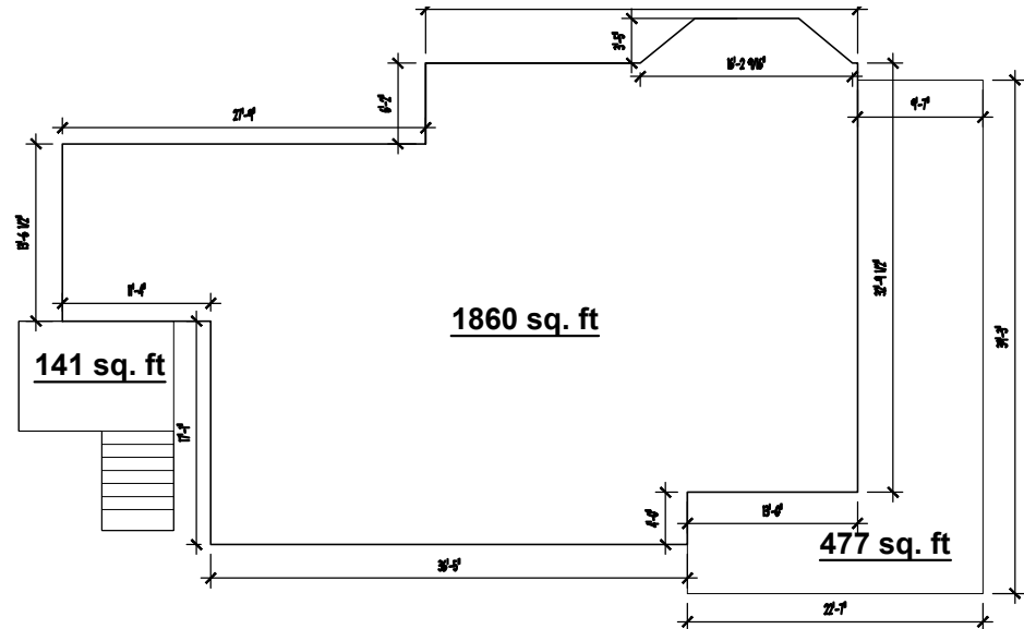
EXISTING MAIN LEVEL PLAN
