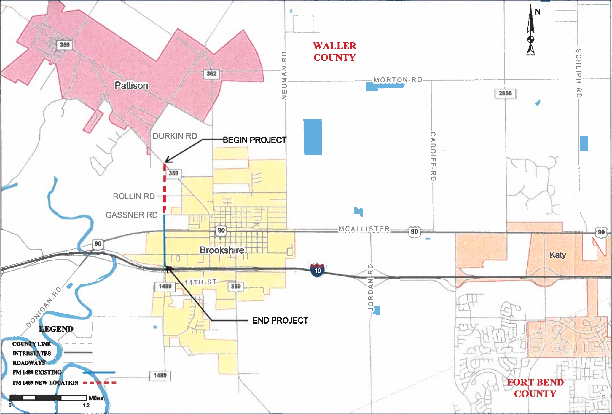
FM 1489 RECONSTRUCT. WIDEN FROM 2 TO LANES BETWEEN I-10 AND FM 359 WITH EXTENSION FROM GASSNER RD TO FM 359. APPROXIMATE LENGTH: 1.9 MILES
