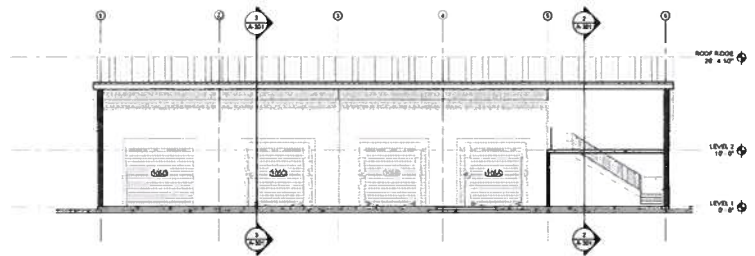
3 BUILDING SECTION 1/8" = 1'-0"
