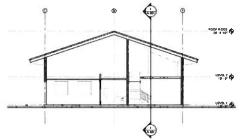
2 BUILDING SECTION 1/8" = 1'-0"
