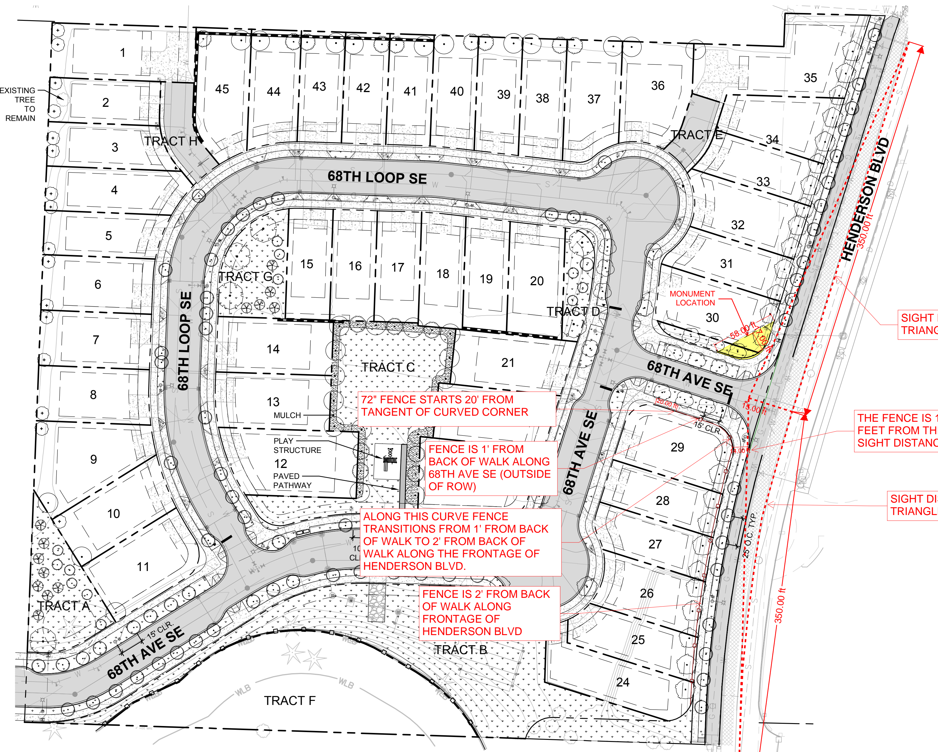
1 LANDSCAPE PLAN
