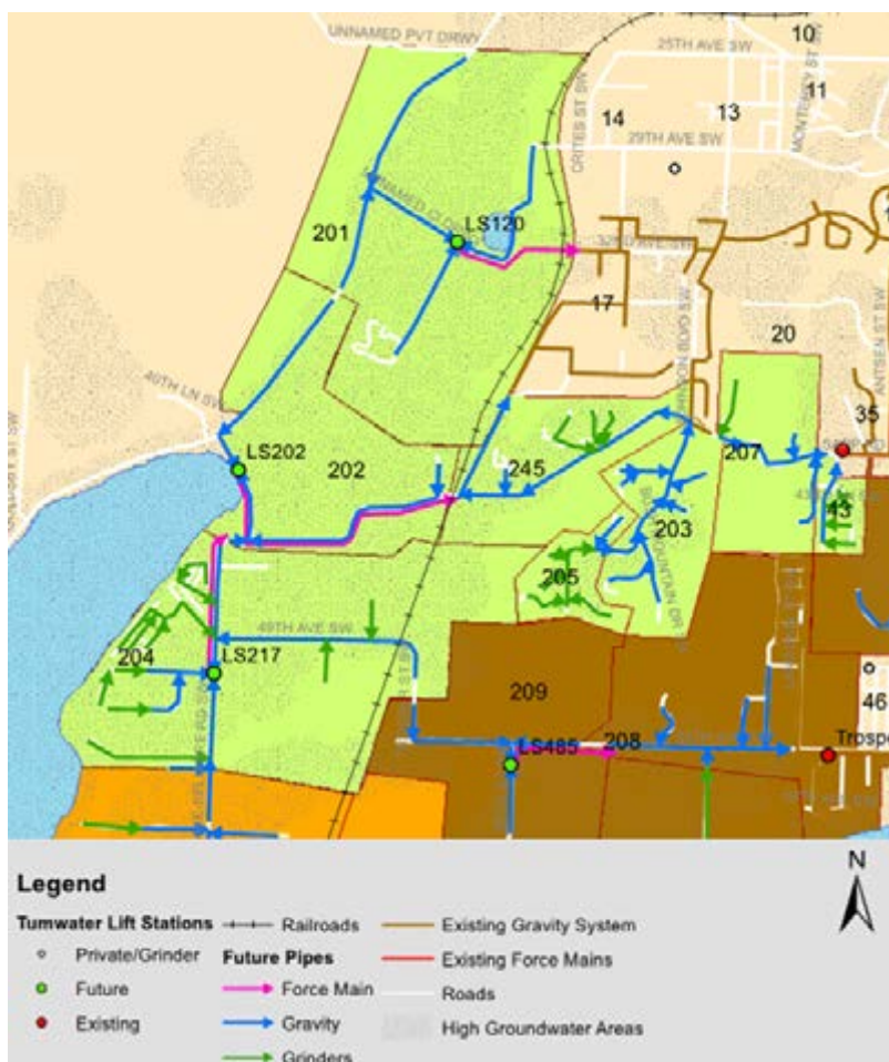
FIGURE 5-6. Recommended sewer servicing for the Mottman Tributary
