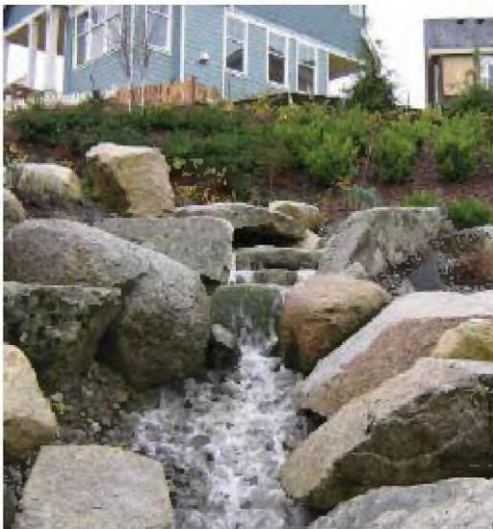
Figure 5.C.4-2. Example now control system incorporated into the site design as an amenity, High Point West, Seattle.
