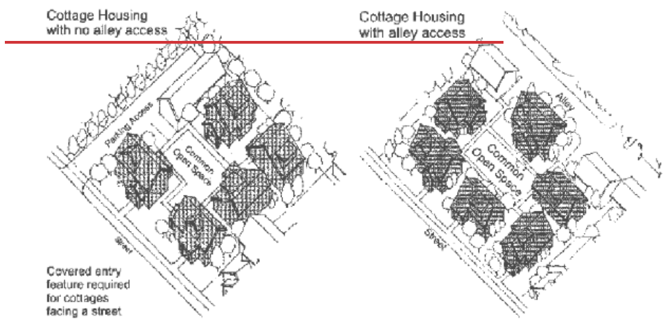
Figure 5.C.1.1. Typical cottage housing layouts.
