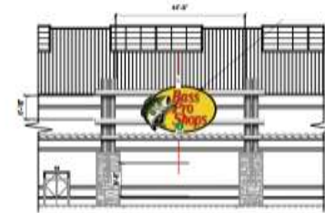
Partial Building Rear Elevation - West Scale: 1/16" = 1'-0"
