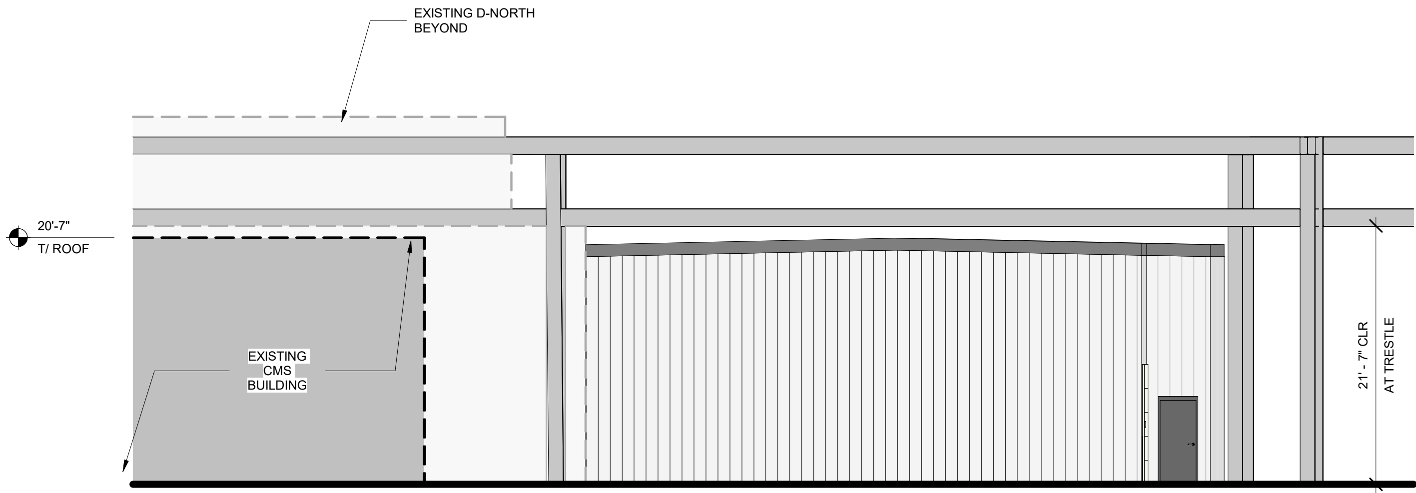
1 FACILITIES STORAGE - NORTH ELEVATION A2.40 1/8" = 1'-0"
