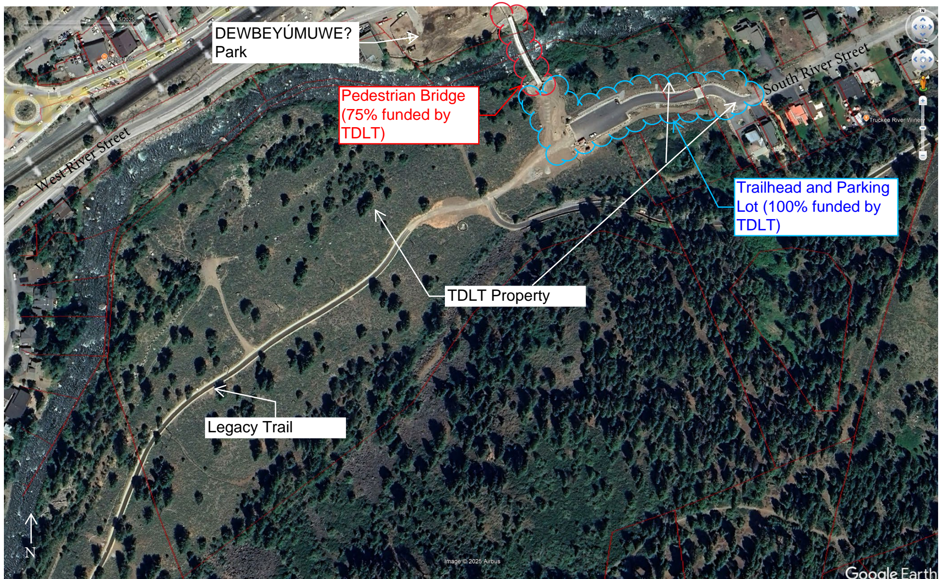
SITE PLAN
