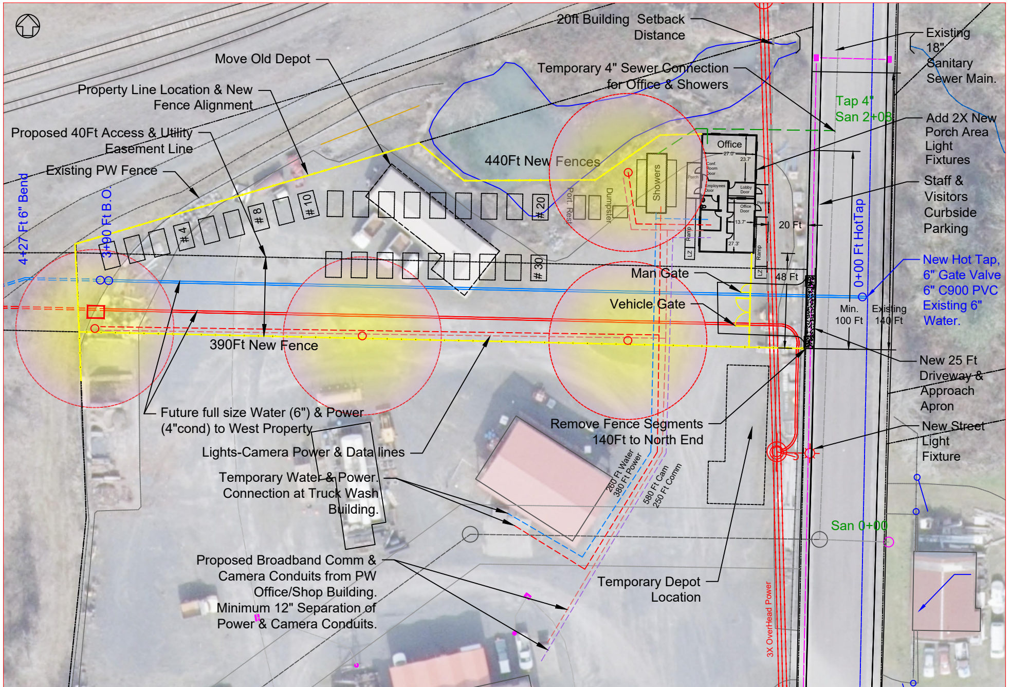
Exhibit "A" 1550 - 24th Avenue Utility Map - Perm Water Power, Lights, & Camera
