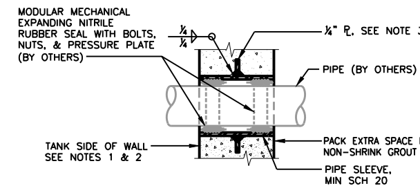
TANK WALL PIPE PENETRATION (DOUBLE LINK SEAL)
