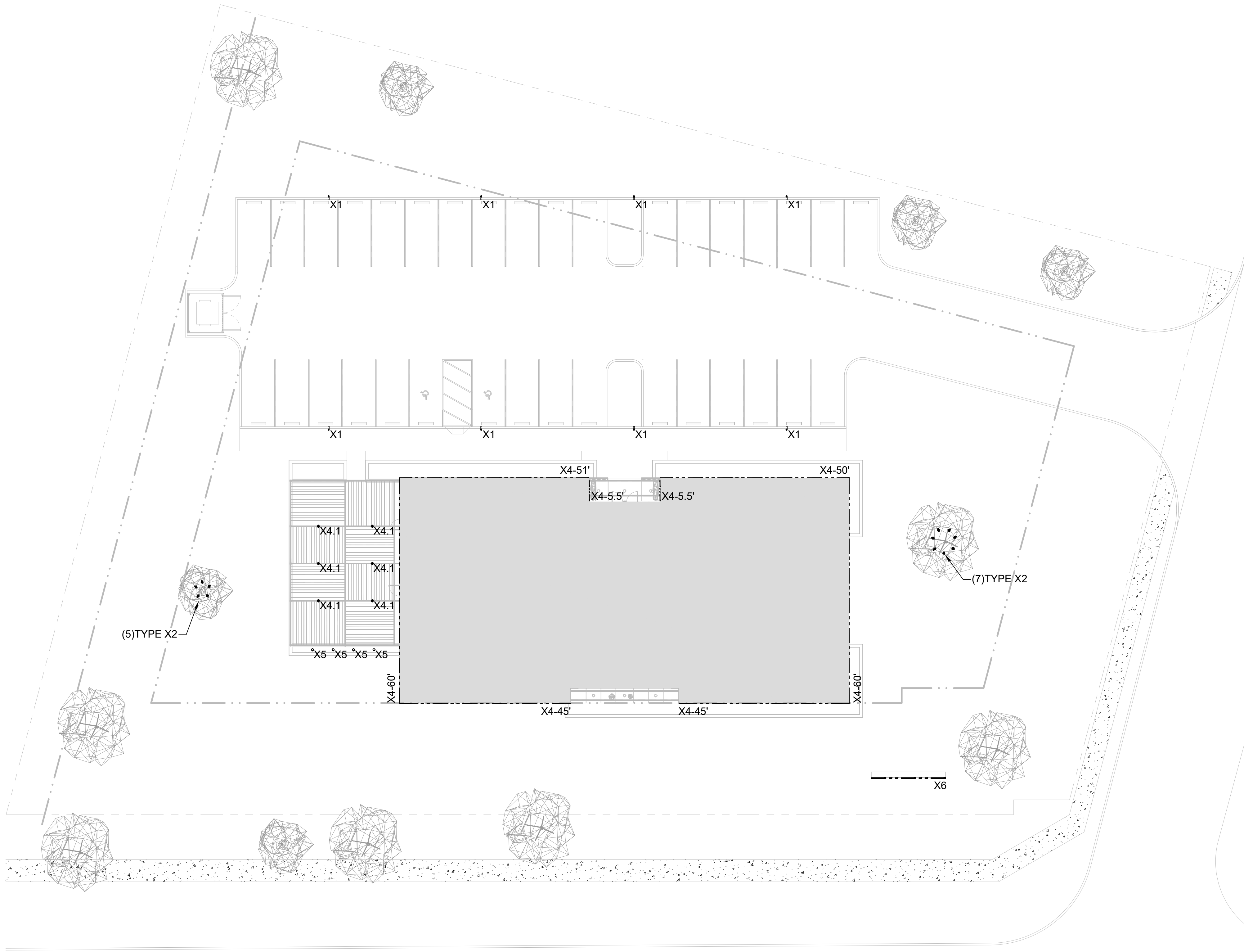
1 PATIO LIGHTING PLAN - OPTION 1 1/16" = 1'-0"
