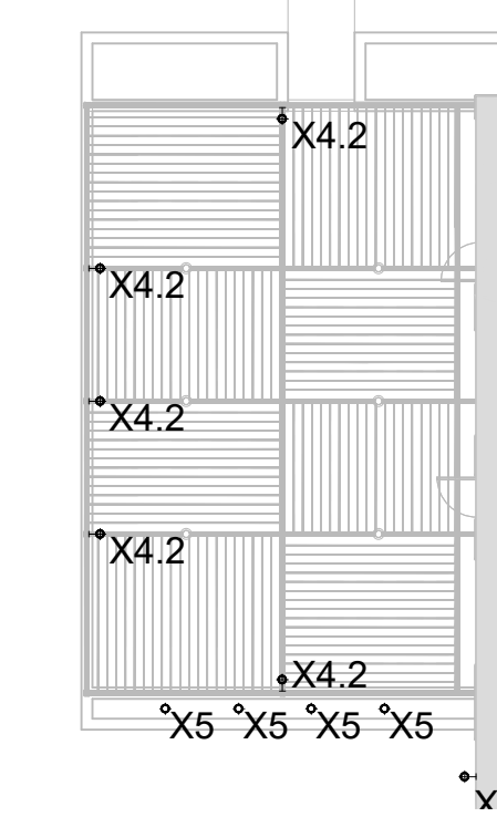
1 PATIO LIGHTING PLAN - OPTION 2 1/16" = 1'-0"
