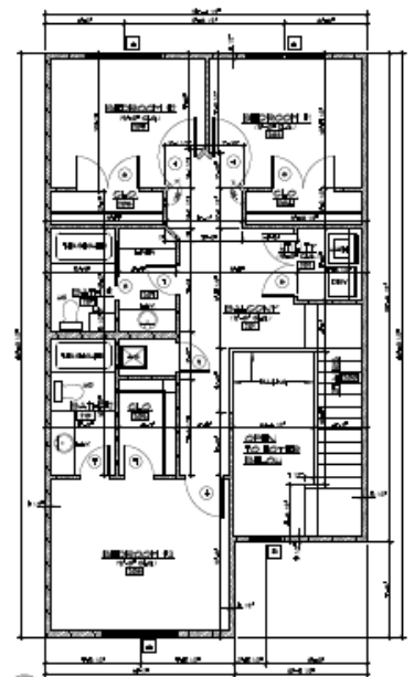
1 UNIT FLOOR PLAN
