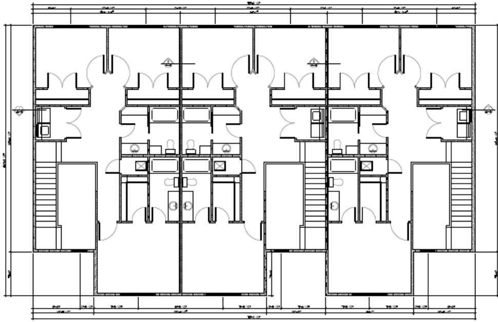
3 UNIT FLOOR PLAN
