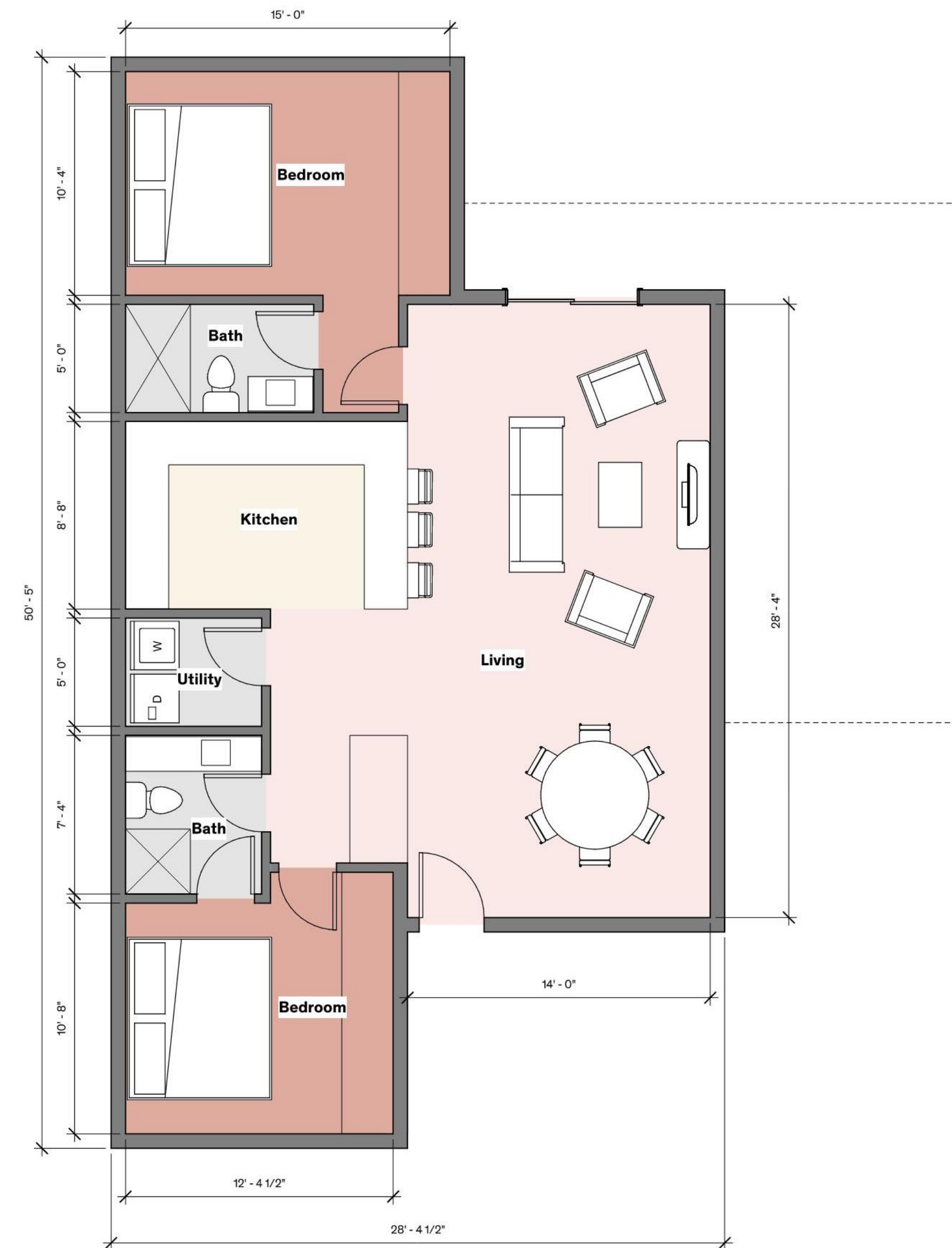
1 2 Bed, 2 Bath - 1020 sq ft \frac{1}{4}" = 1'-0"
