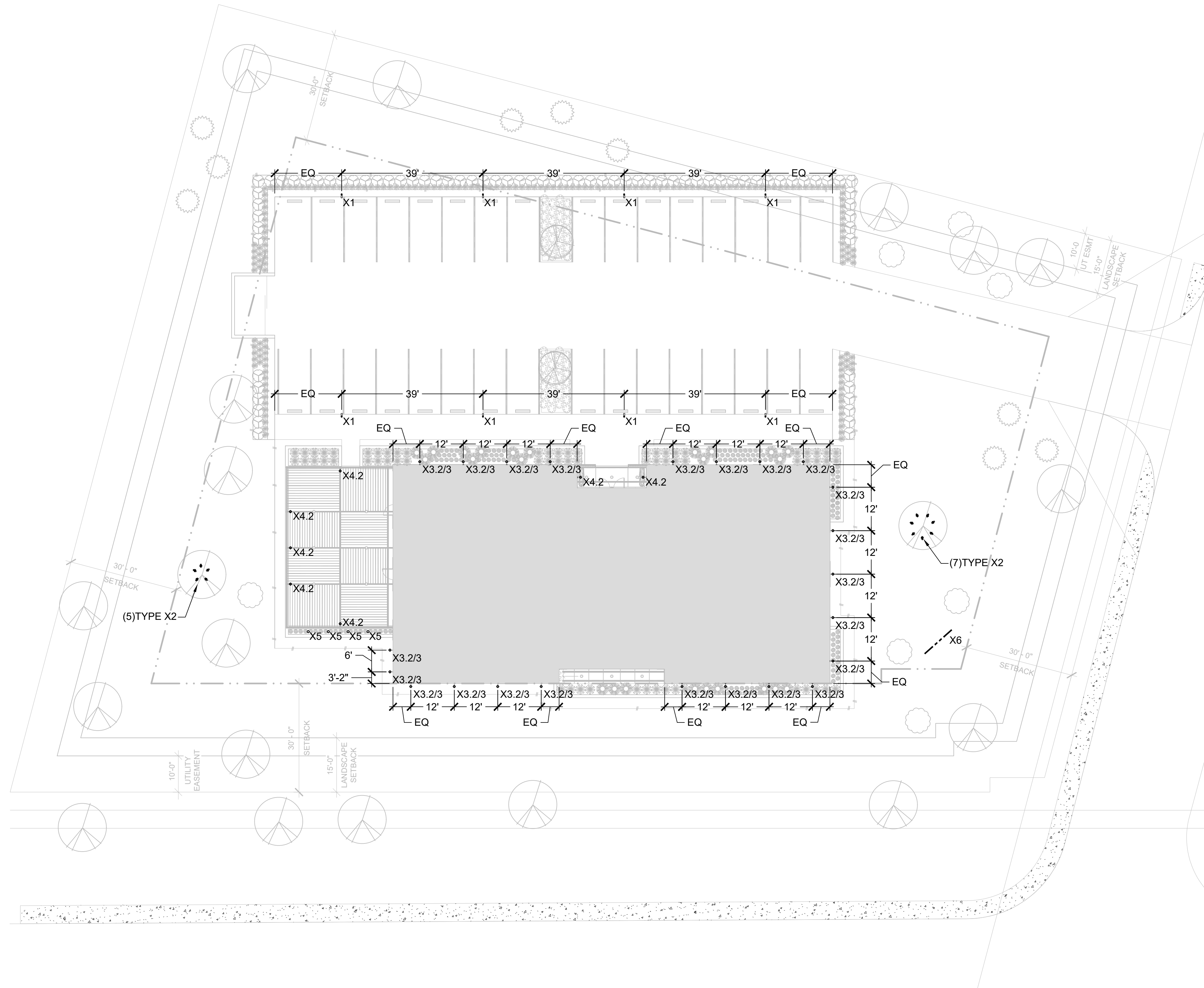
① SITE LIGHTING PLAN - BUILDING FACADE OPTION 2 1/16" = 1'-0"
