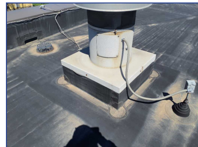
Membrane Shrinkage
