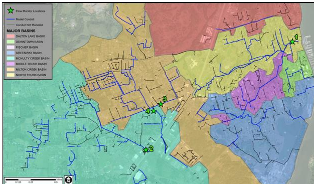
FIGURE 4-1: FLOW MONITORING LOCATIONS
