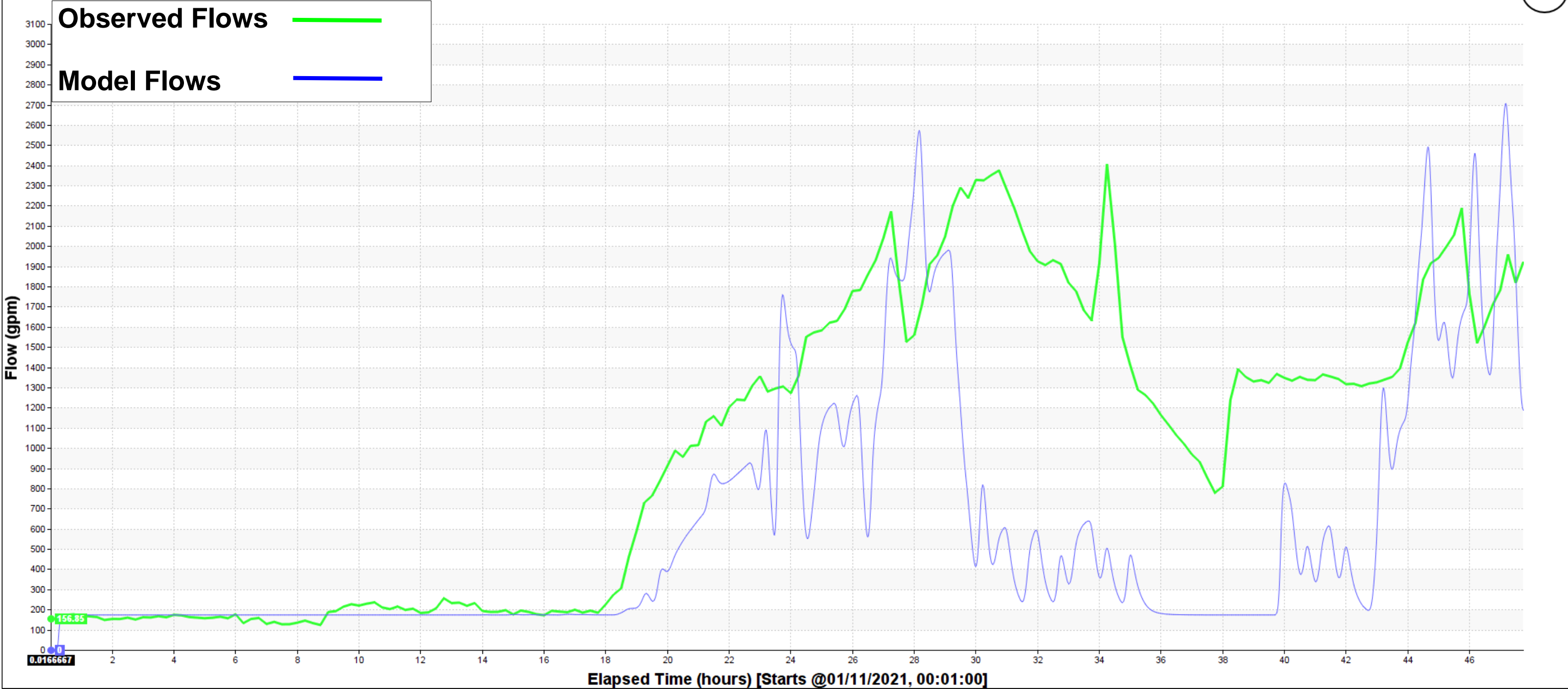
Conduit SW-1034 (Run/Measured Volumes : 223473.01 / 384930.55 ft3)
