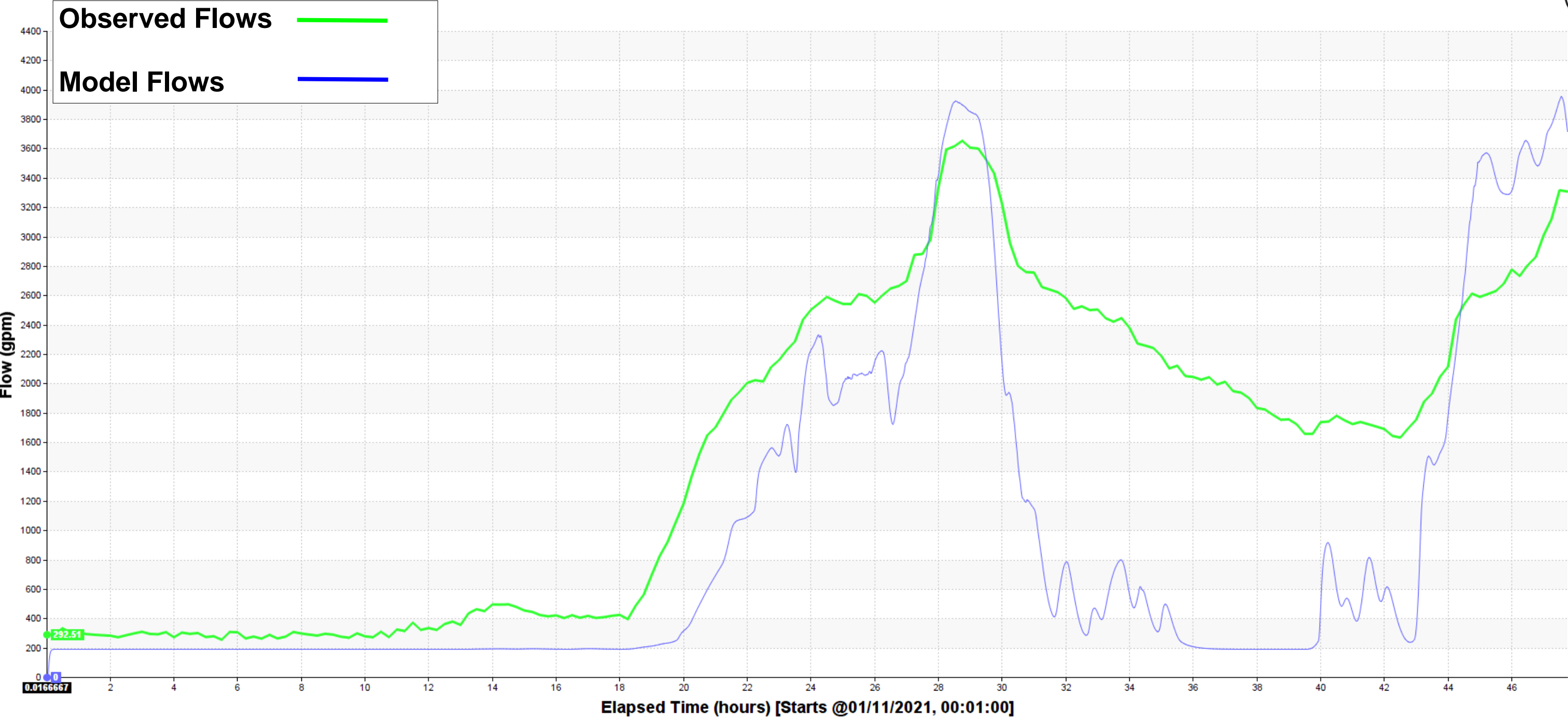
Conduit SW-1614 (Run/Measured Volumes : 359974.83 / 583531.57 ft3)
