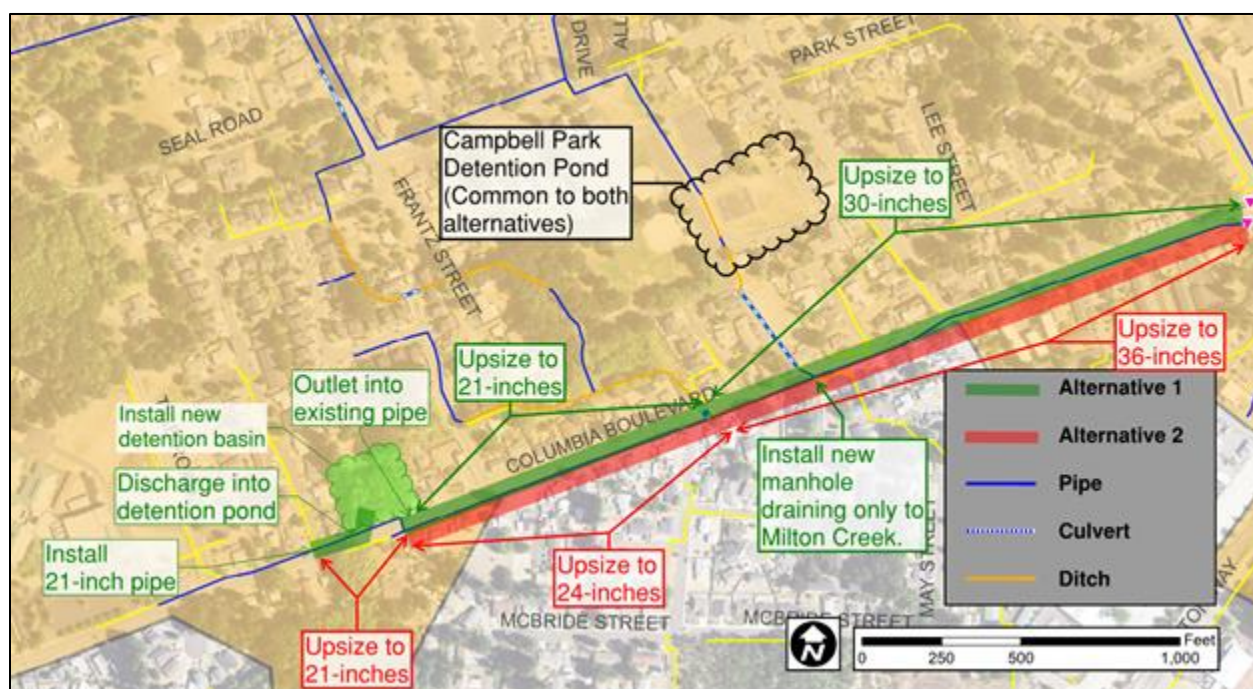
FIGURE 6-11: MILTON CREEK ALTERNATIVES
