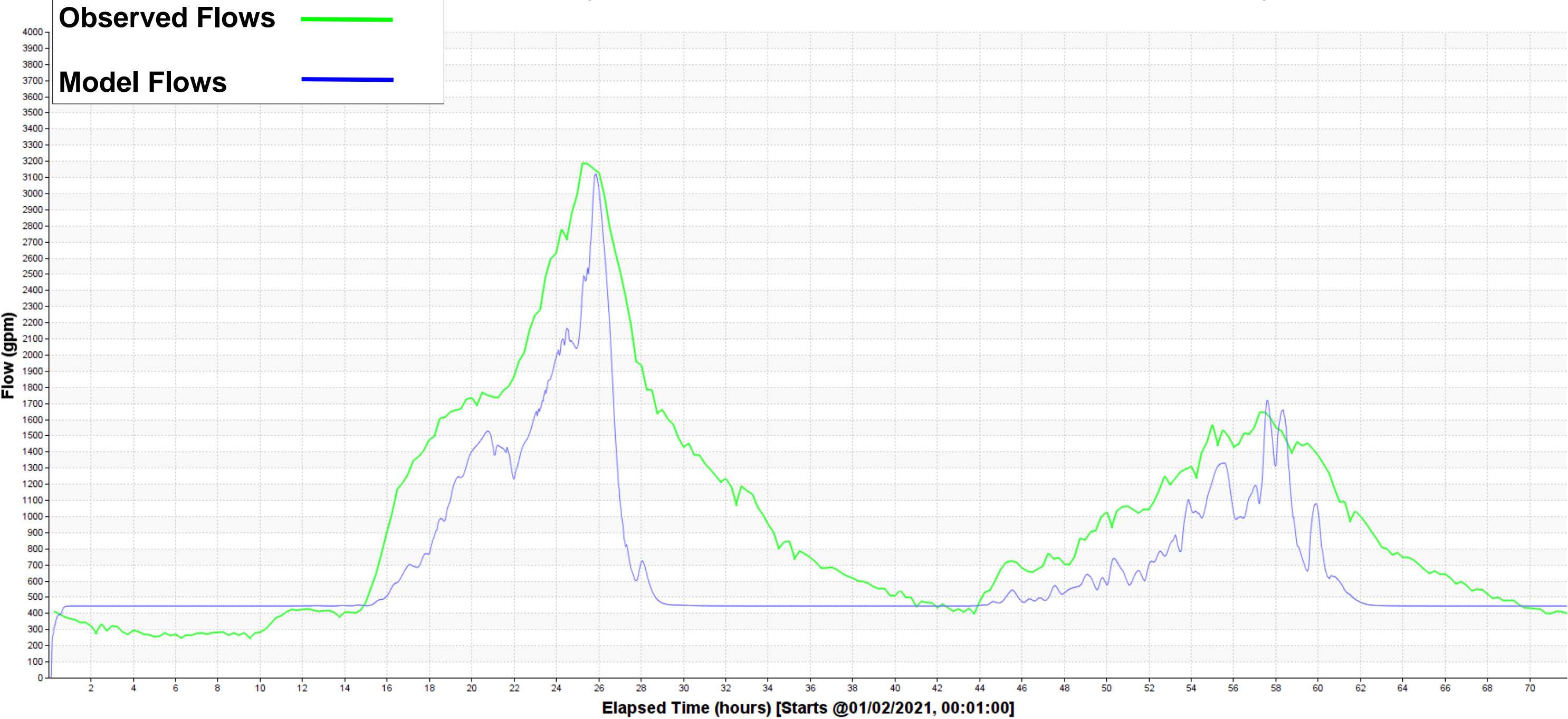
Conduit SW-1364 (Run/Measured Volumes : 402626.89 / 562761.91 ft3)
