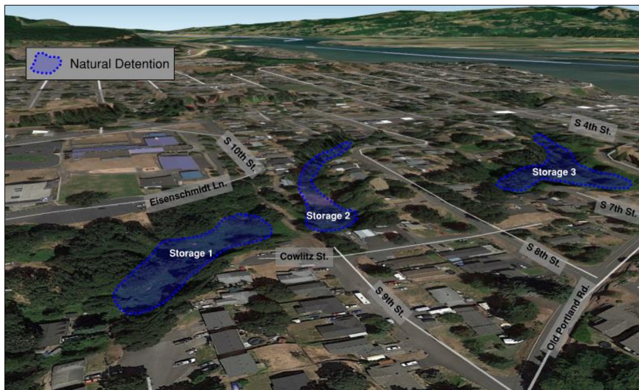
FIGURE 6-4: MIDDLE TRUNK NATURAL DETENTION STORAGE LOCATIONS
