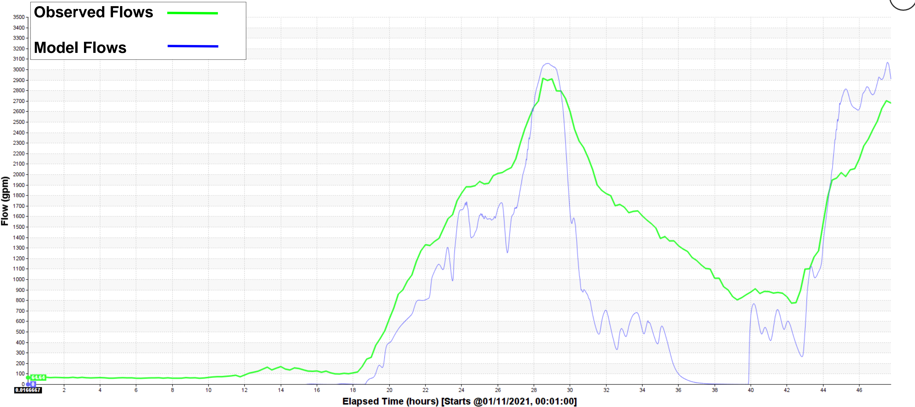
Conduit SW-1364 (Run/Measured Volumes : 260166.84 / 383876.69 ft3)
