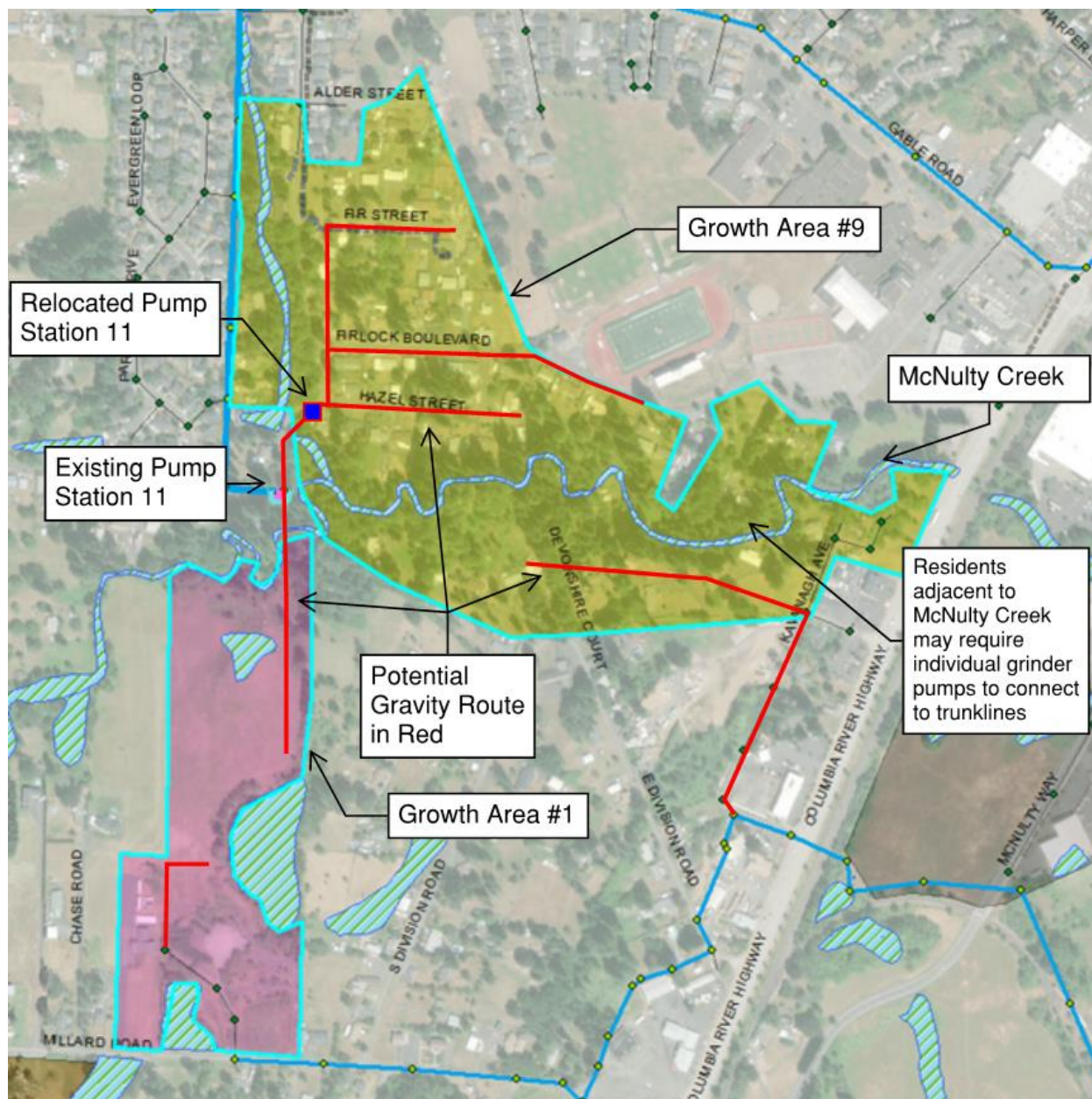
FIGURE 5-5: GROWTH AREA #1 AND #9 PROPOSED WASTEWATER INFRASTRUCTURE
