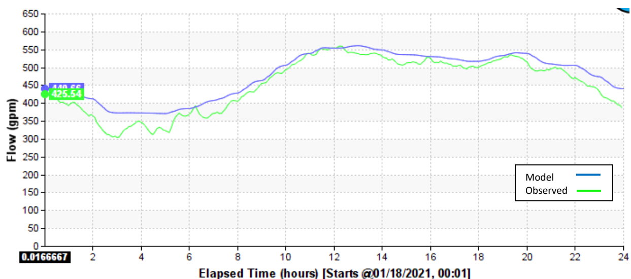
CHART 4-1: SAMPLE BASE FLOW CALIBRATION SITE 3
