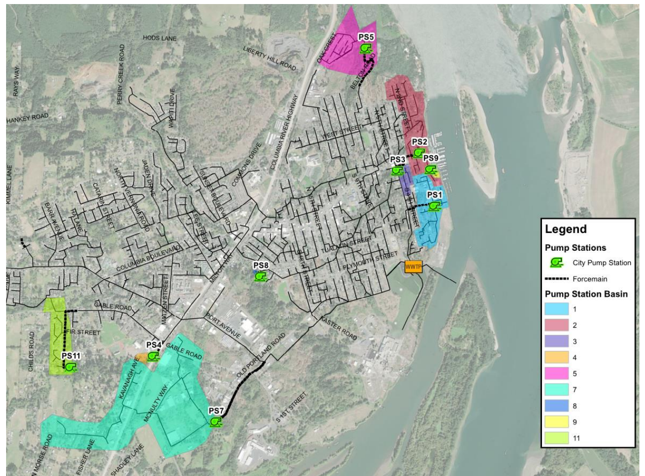
FIGURE 3-1 – EXISTING PUMP STATION BASINS
