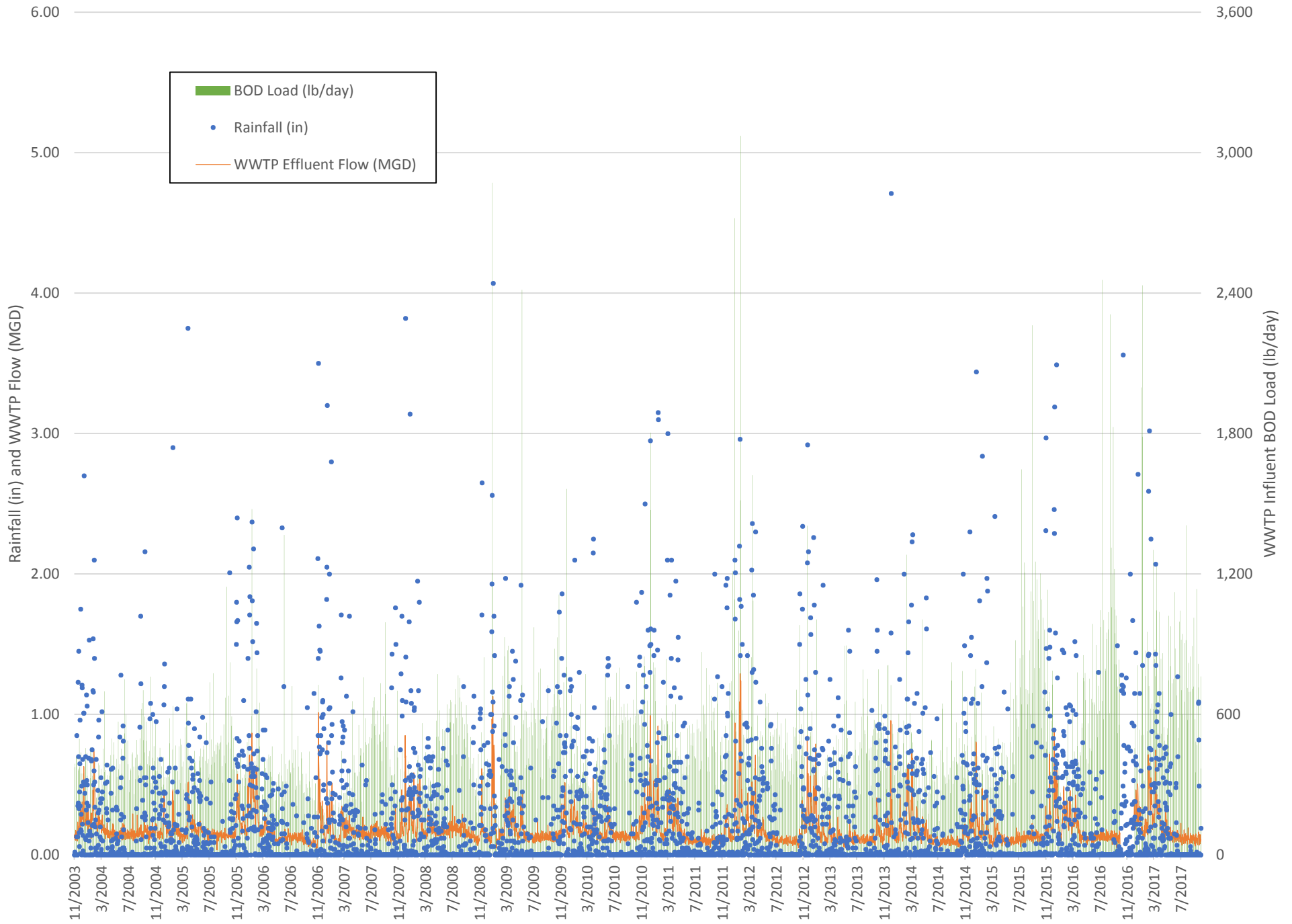
Rainfall, WWTP Effluent Flow, and WWTP Influent BOD Load, Nov 2003 to Sep 2017
