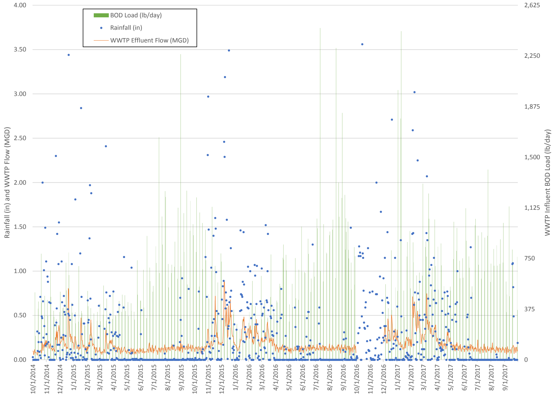
Rainfall, WWTP Effluent Flow, and WWTP Influent BOD Load - Oct 2014 to Sep 2017
