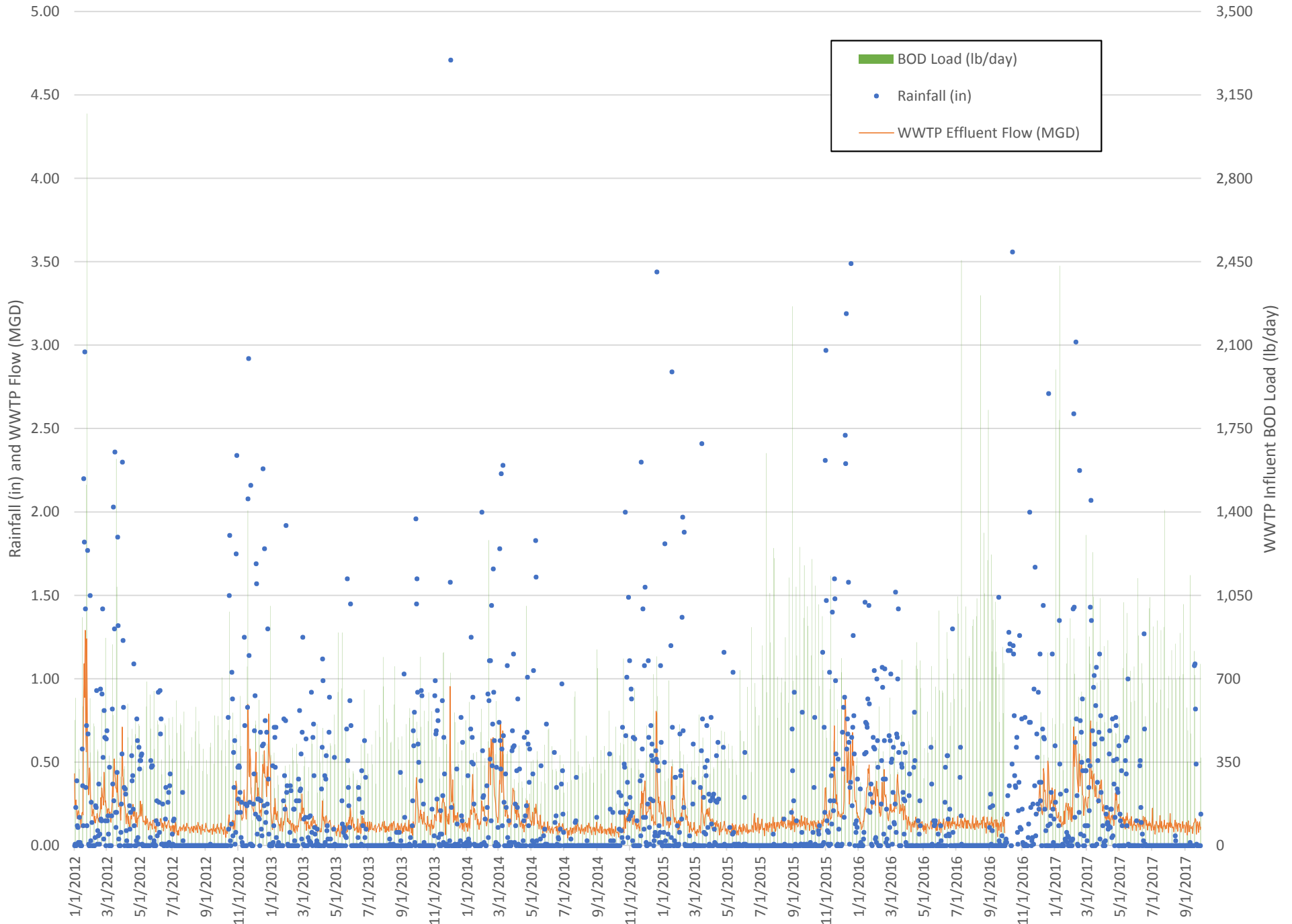
Rainfall, WWTP Effluent Flow, and WWTP Influent BOD Load, Jan 2012 to Sep 2017
