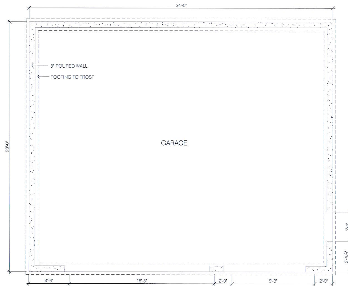
① FOUNDATION PLAN SCALE: 1/4"=1'-0"
