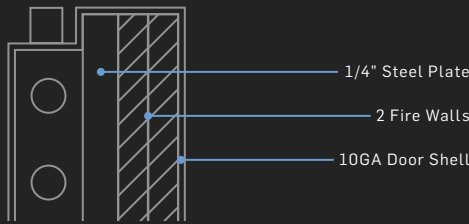
DOOR STEEL THICKNESS
