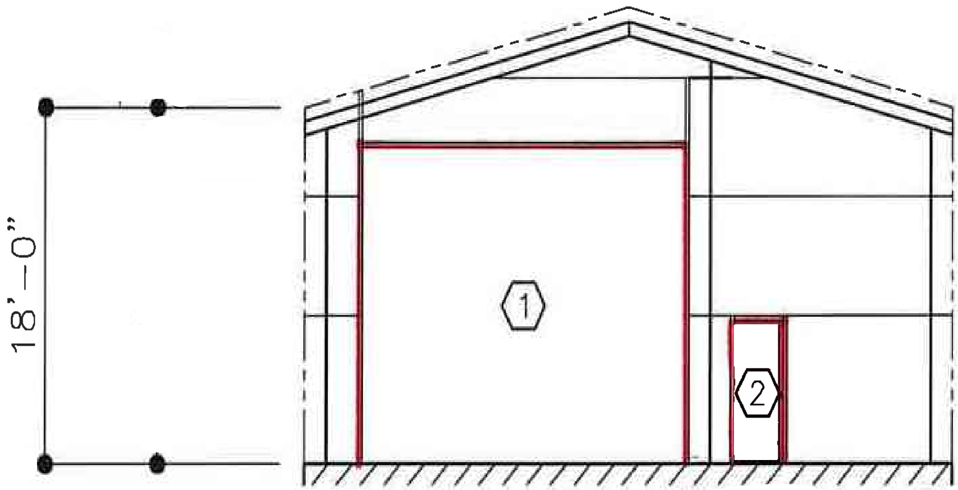
South Elevation
