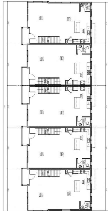
2 SPLEX - LEVEL 2 - 3 STORY A10 SCALE 1/8" = 1'-0"
