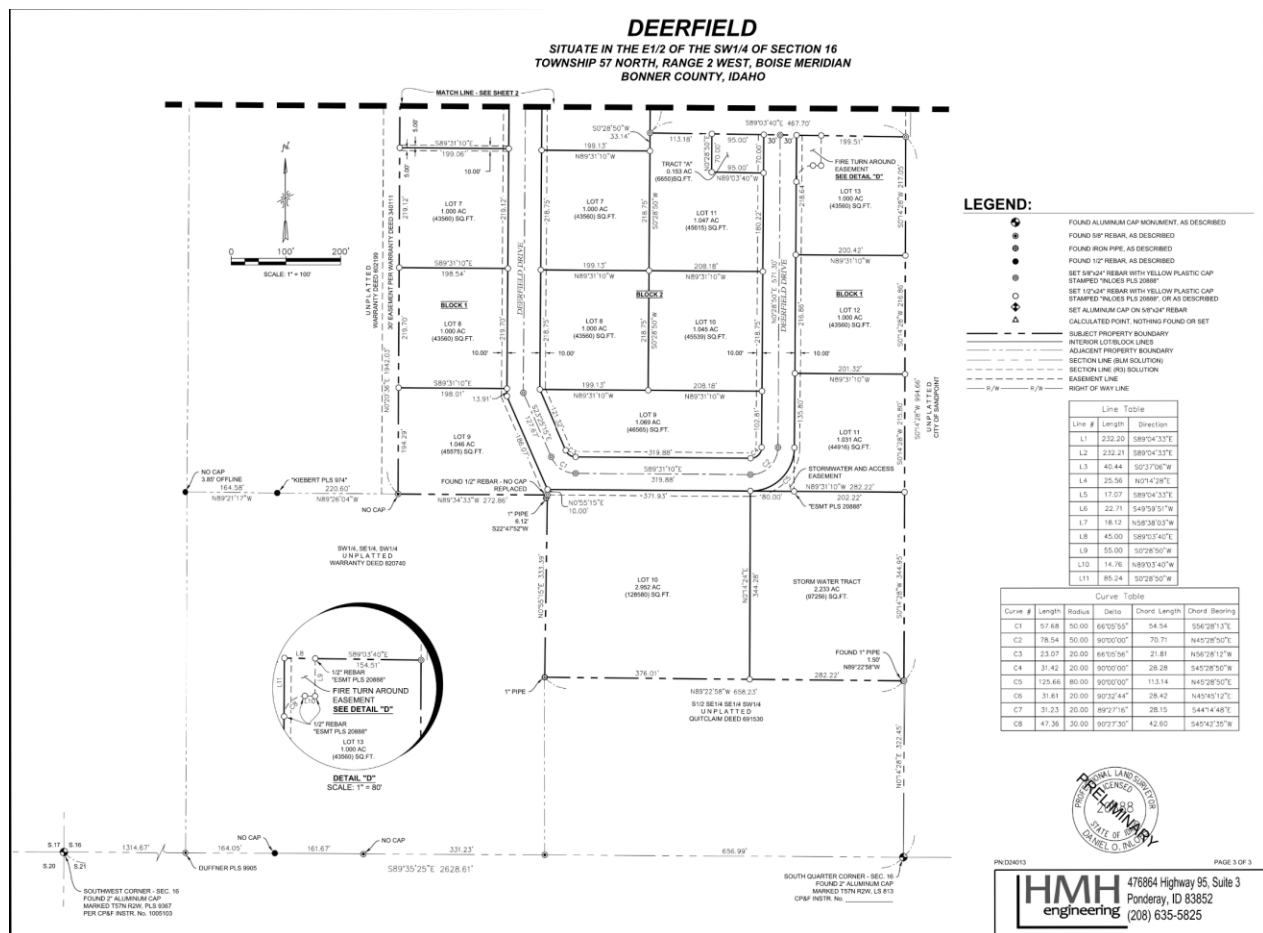
Figure 3 - Preliminary Plat
