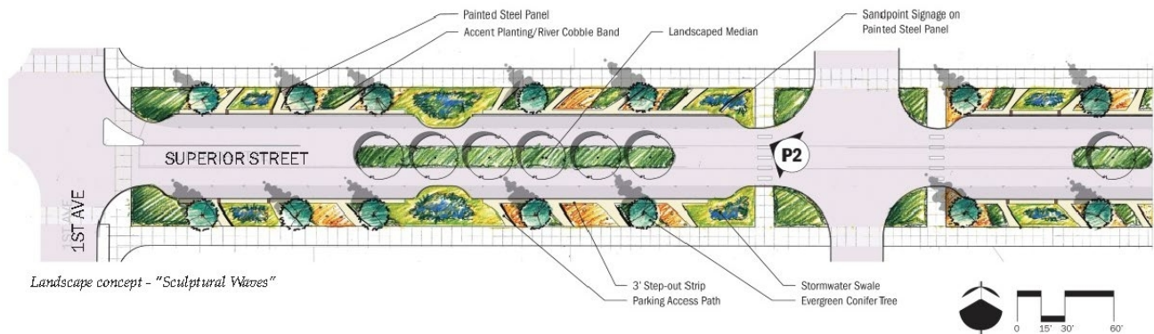
Figure 11 Concepts for Superior Street from the Downtown Streets Plan and Design Guide
