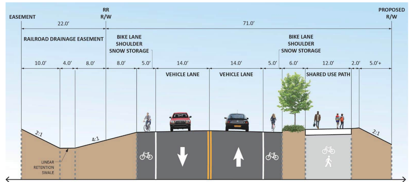
GREAT NORTHERN ROAD SECTION A-A
