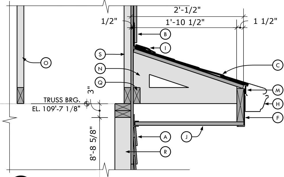
2 END WALL EAVE DETAIL A/6 SCALE: 1" = 1'-0" (AT ORIG. SHEET SIZE)
