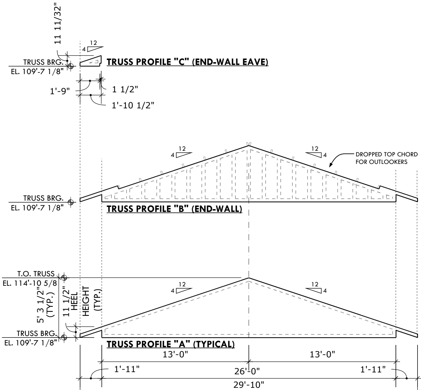
1 TRUSS PROFILES SCALE: 3/16" = 1'-0" (AT ORIG. SHEET SIZE)
